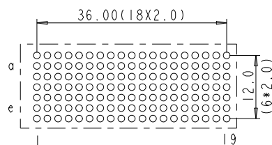
LAY-OUT P.C.B. - HOLE (FRONT SIDE)
