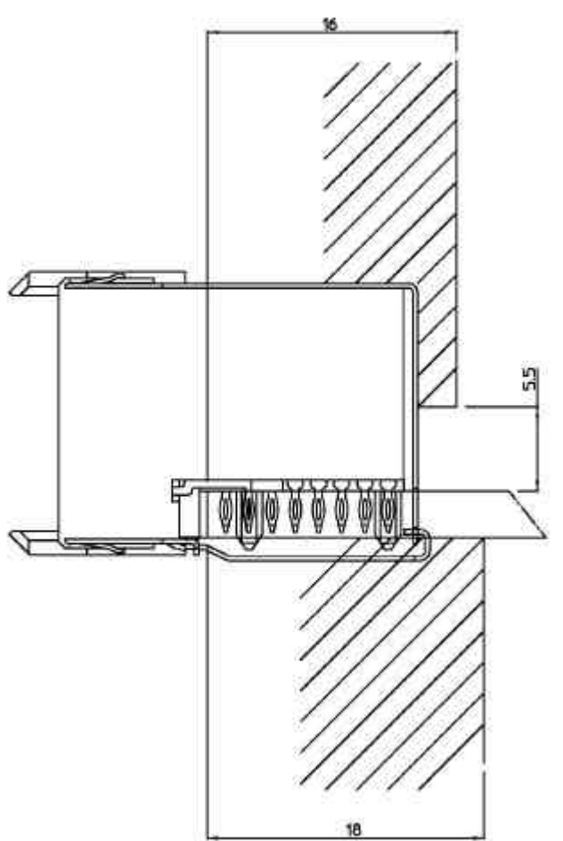
Figure 7 -- Keep-out Zones
