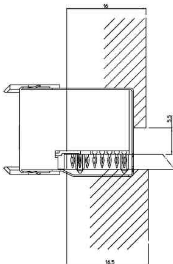
Figure 6 -- Keep-out Zones
