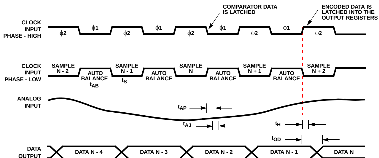
FIGURE 1. INPUT-TO-OUTPUT TIMING
