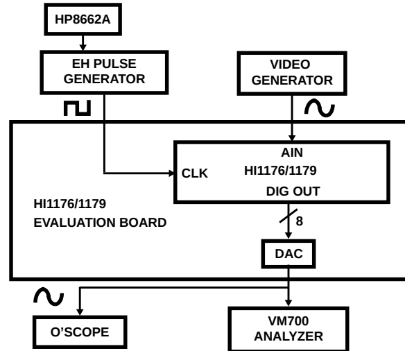
FIGURE 7. VIDEO TEST SYSTEM
