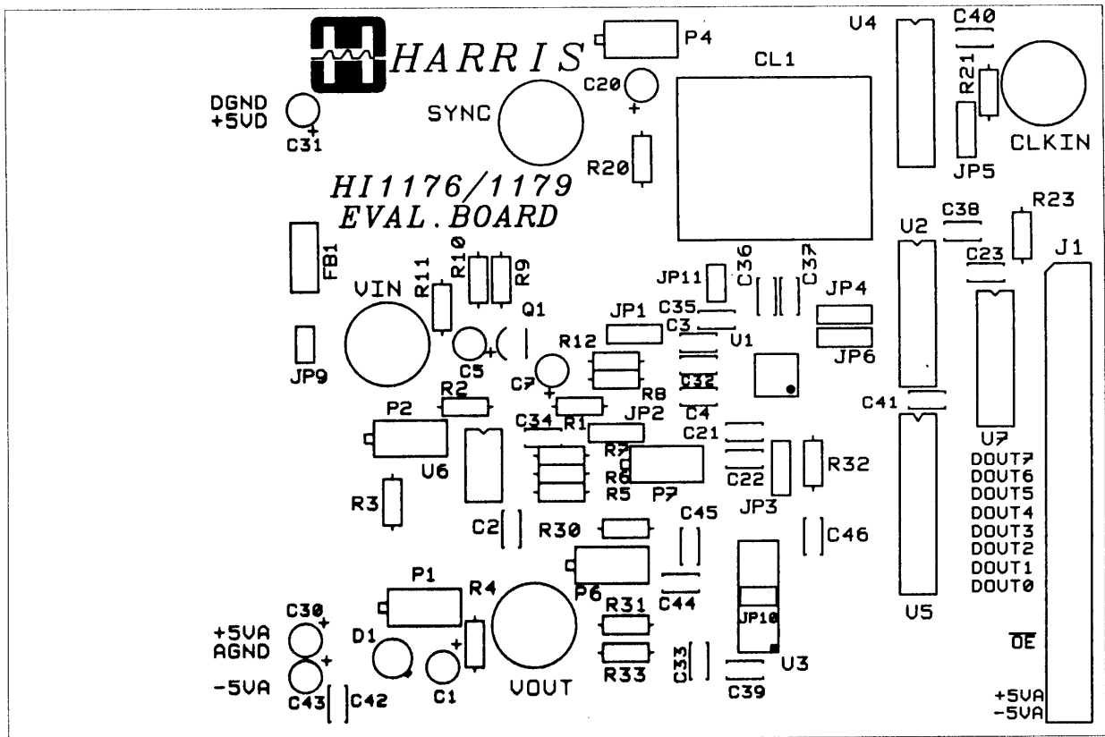
FIGURE 13. SILKSCREEN
