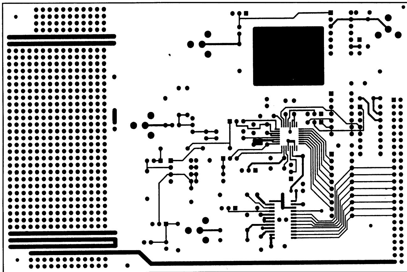
FIGURE 9. COMPONENT SIDE
