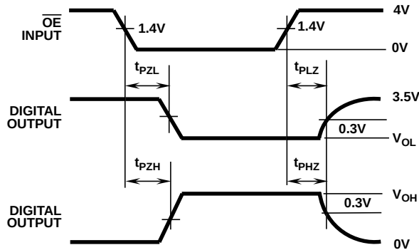
FIGURE 4. ENABLE/DISABLE TIMING
