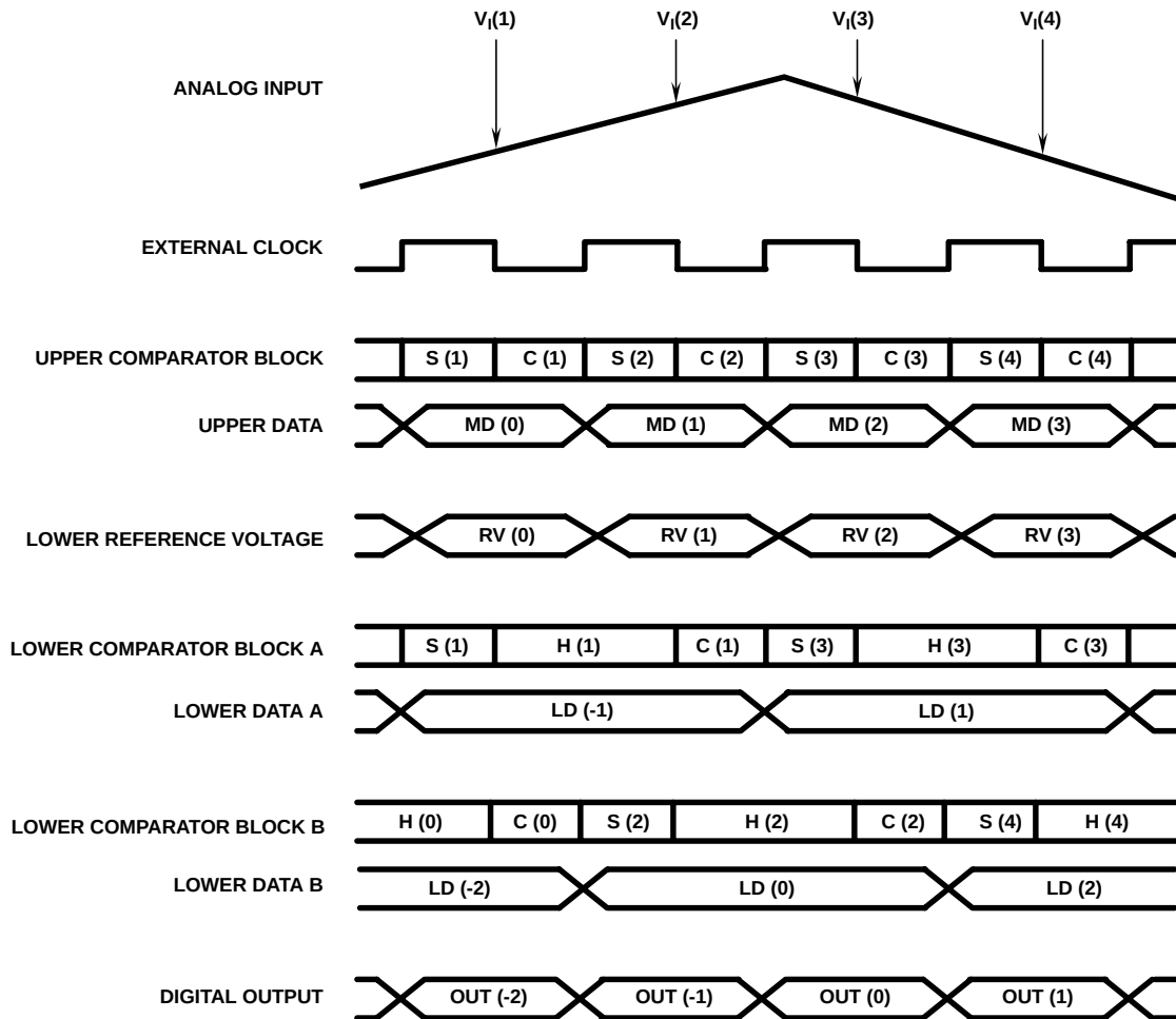
FIGURE 3. HI1176/HI1179 TIMING
