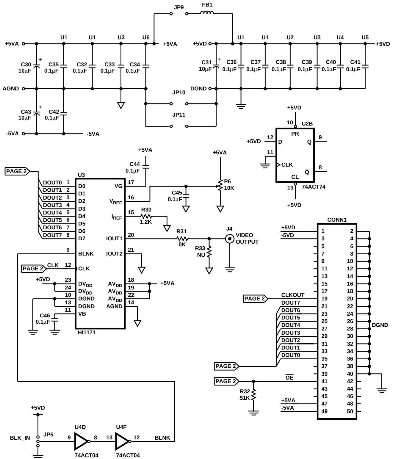
FIGURE 16. SCHEMATIC
