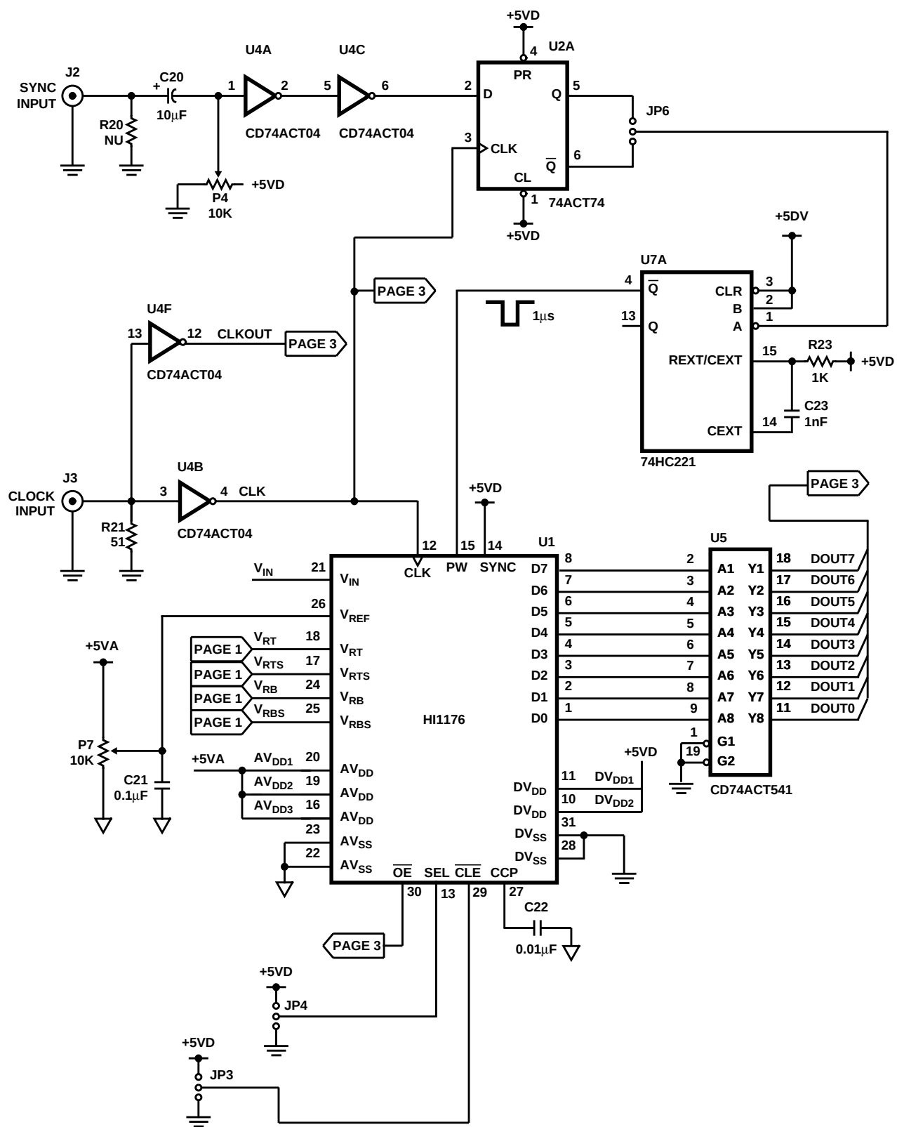
FIGURE 15. SCHEMATIC
