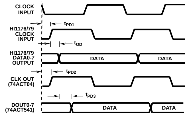
FIGURE 5. INPUT-TO-OUTPUT TIMING
