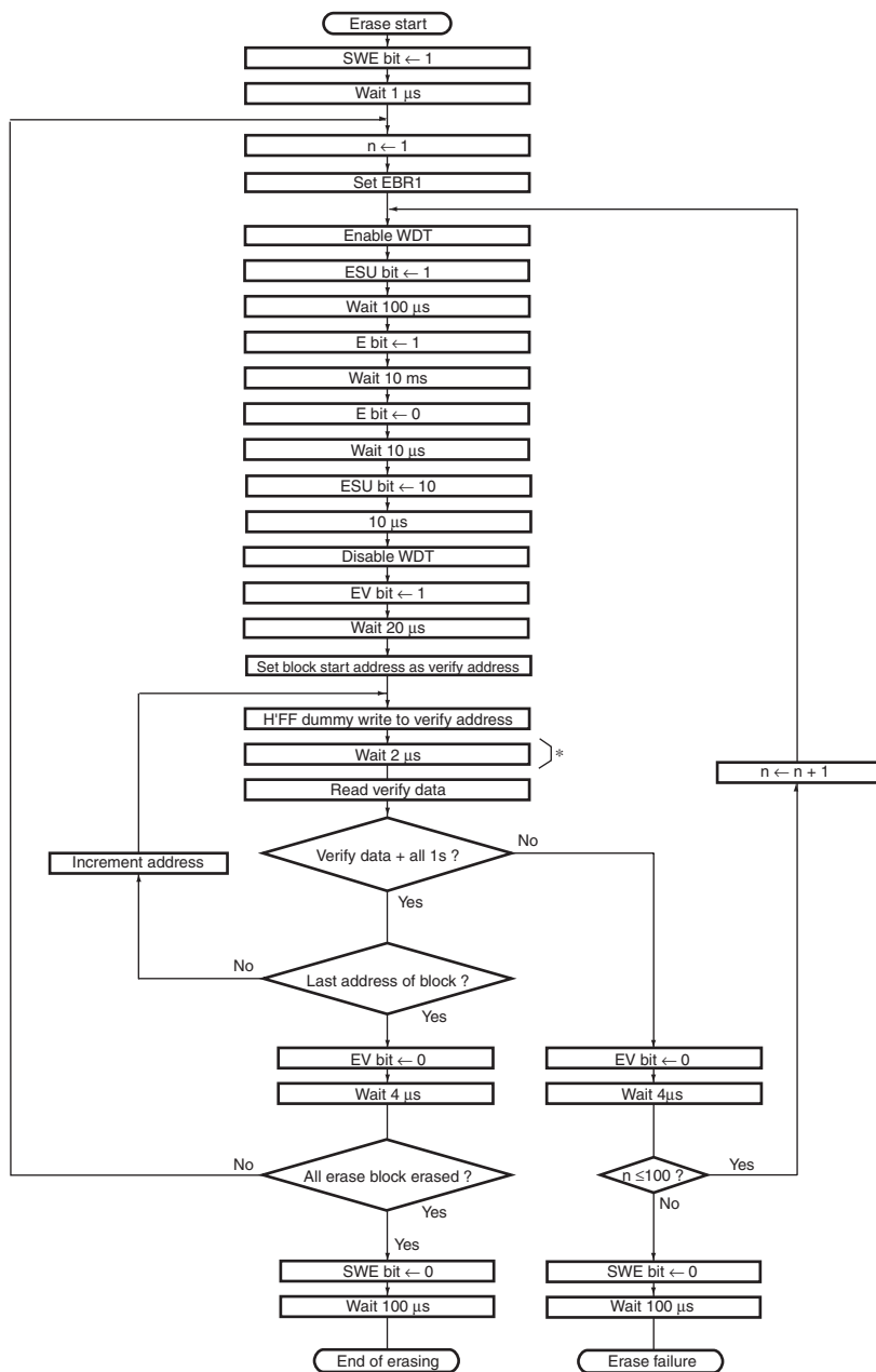
Figure 7.4 Erase/Eraser-Verify Flowchart
