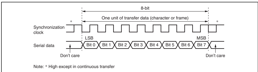
Figure 14.10 Data Format in Clocked Synchronous Communication
