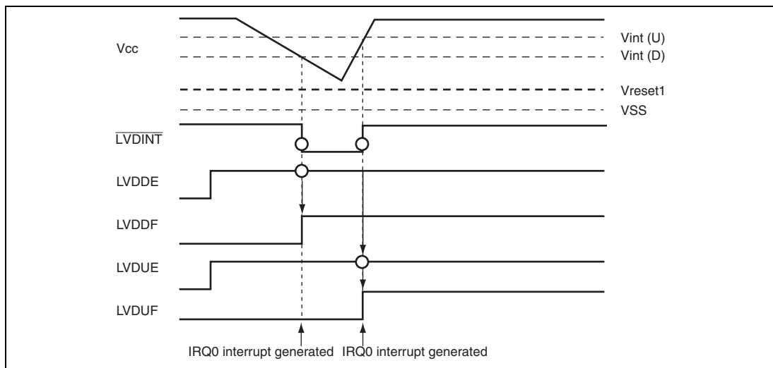
Figure 17.5 Operational Timing of LVDI Circuit
