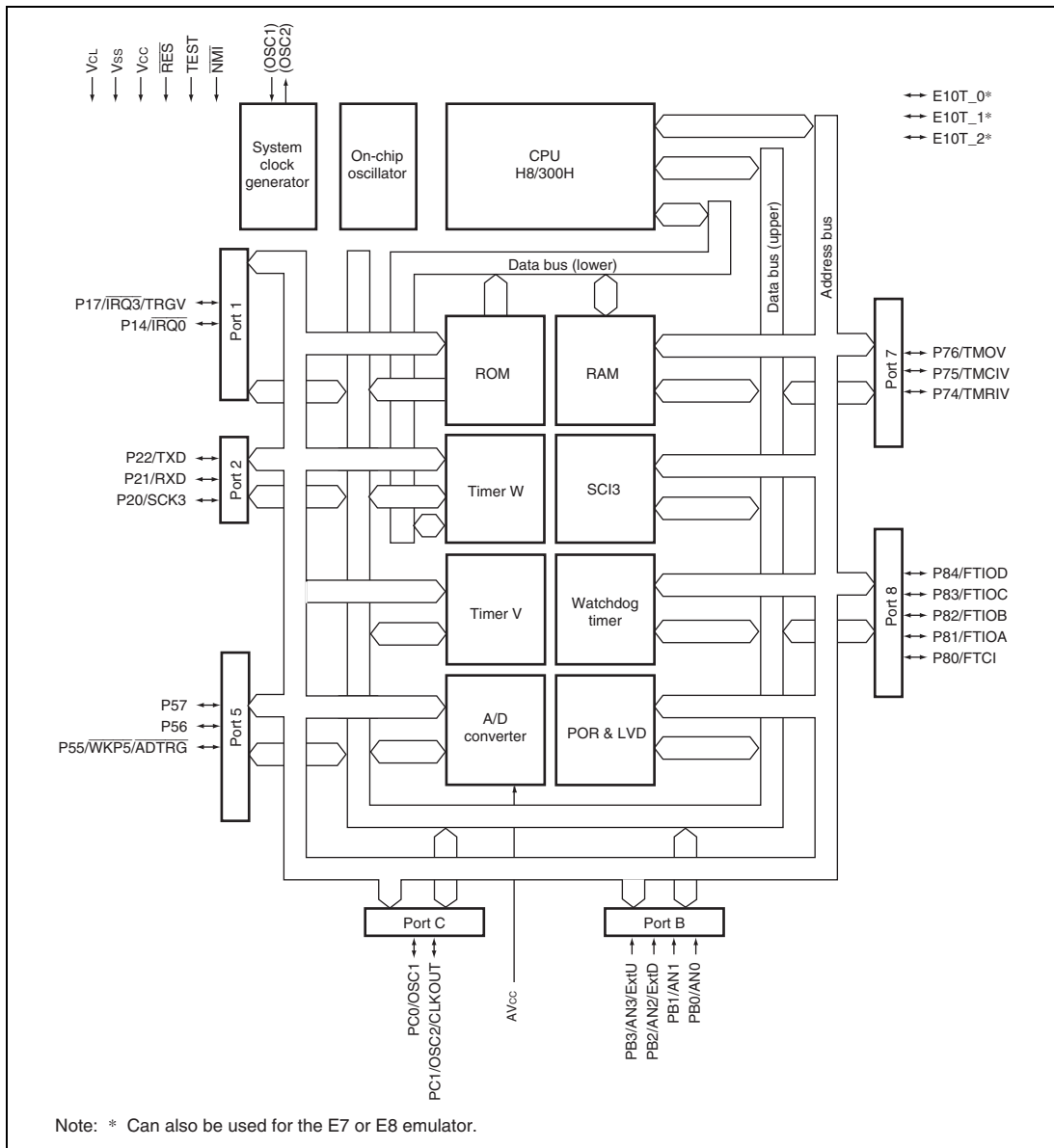
Figure 1.2 Internal Block Diagram of H8/36902 Group
