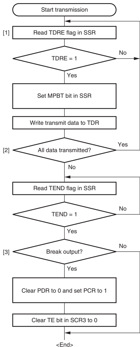
Figure 14.17 Sample Multiprocessor Serial Transmission Flowchart
