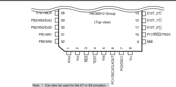
Figure 1.3 Pin Arrangement of H8/36912 Group (FP-32A)
