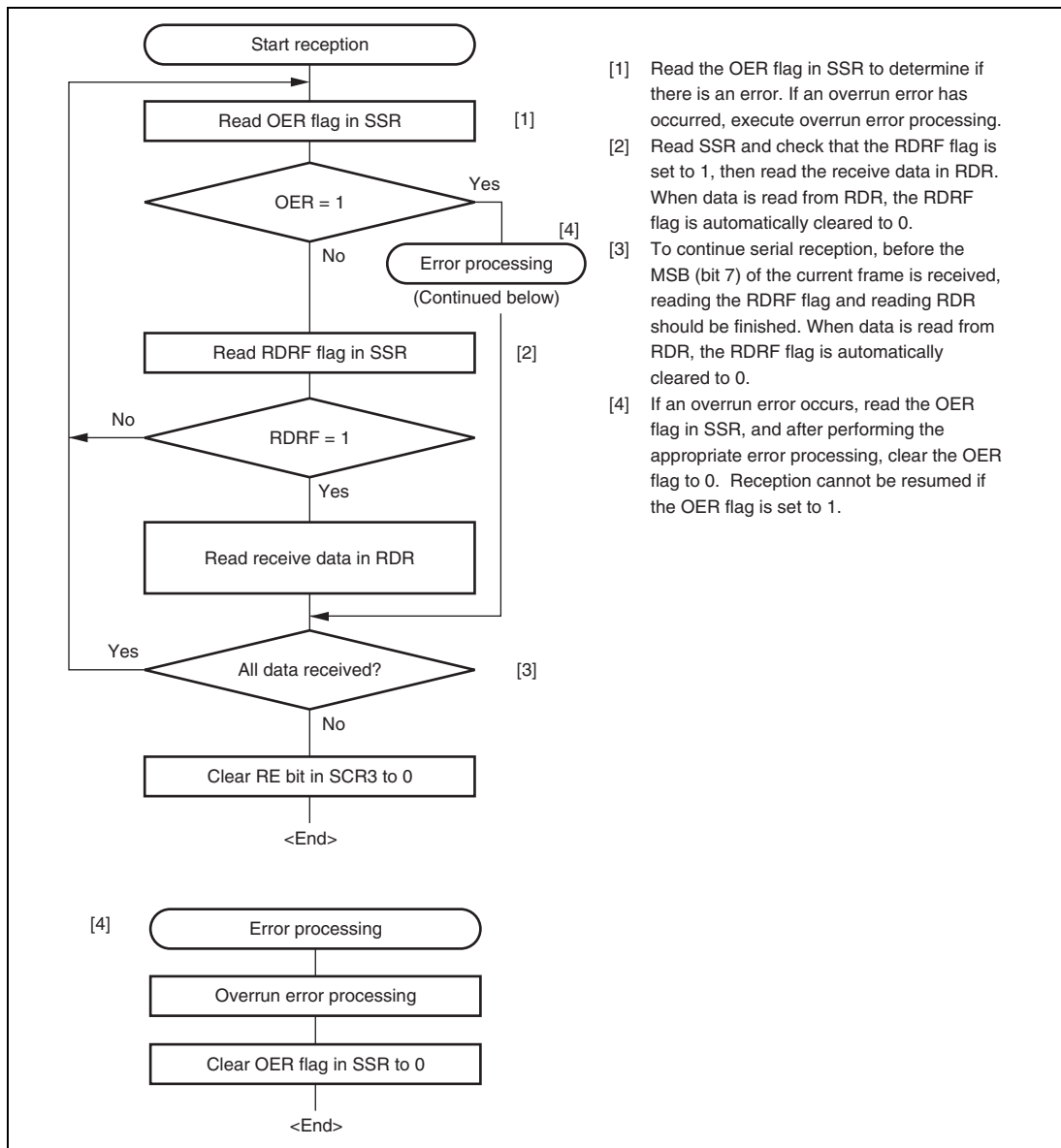
Figure 14.14 Sample Serial Reception Flowchart (Clocked Synchronous Mode)
