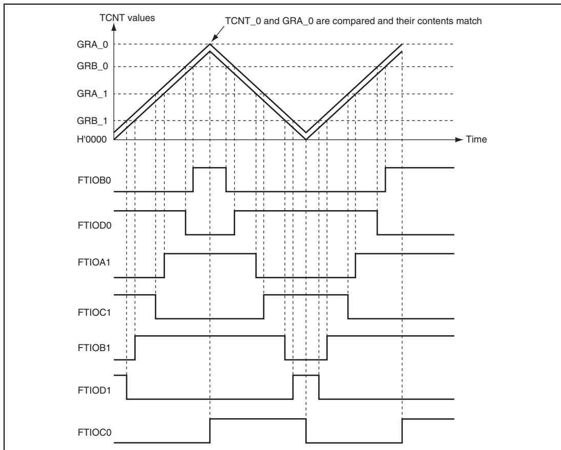
Figure 14.31 Example of Complementary PWM Mode Operation (1)
