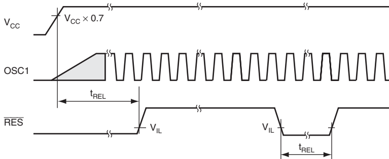
Figure 23.2 \overline{\text{RES}} Low Width Timing
