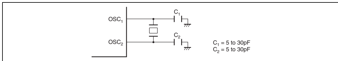
Figure 5.5 Typical Connection to Ceramic Resonator
