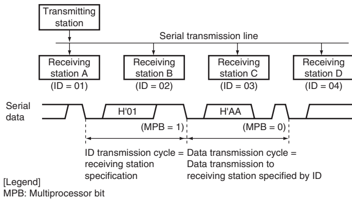
Figure 17.15 Example of Inter-Processor Communication Using Multiprocessor Format (Transmission of Data H'AA to Receiving Station A)
