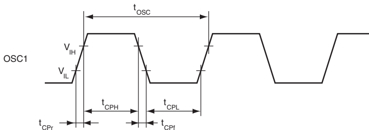
Figure 23.1 System Clock Input Timing
