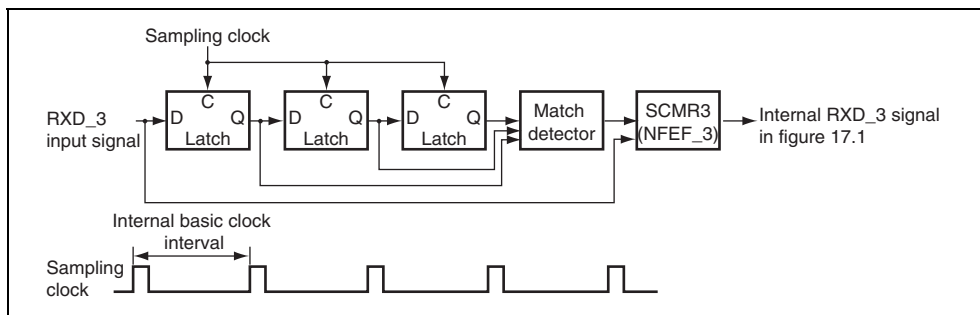
Block Diagram of Noise Canceller
