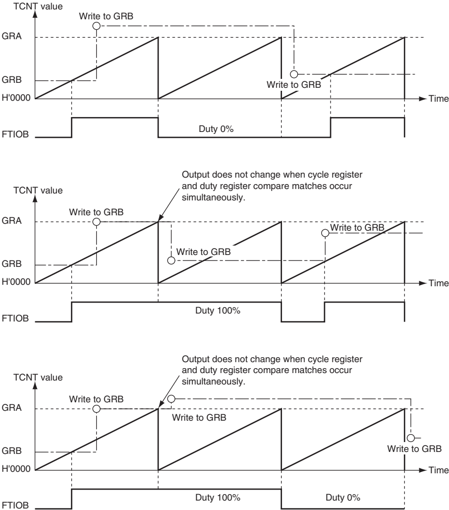
Figure 13.12 PWM Mode Example (TOB = 0, TOC = 0, TOD = 0: Initial Output Values are Set to 0)
