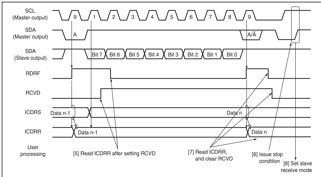
Figure 18.8 Master Receive Mode Operation Timing (2)
