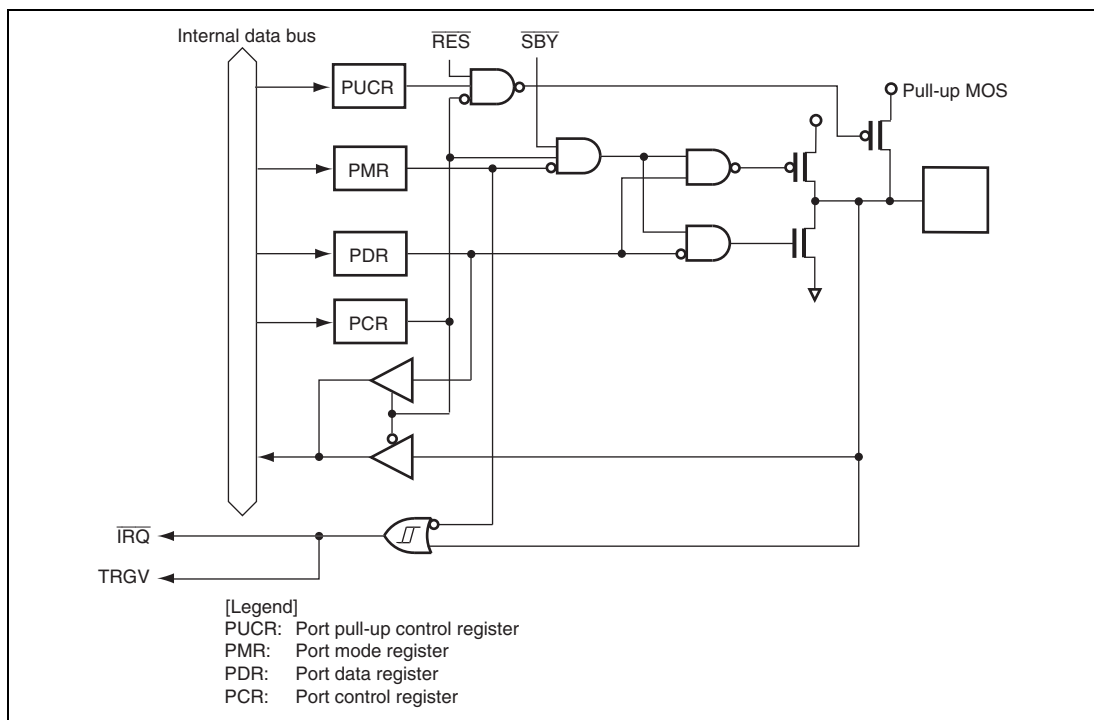
Figure B.1 Port 1 Block Diagram (P17)
