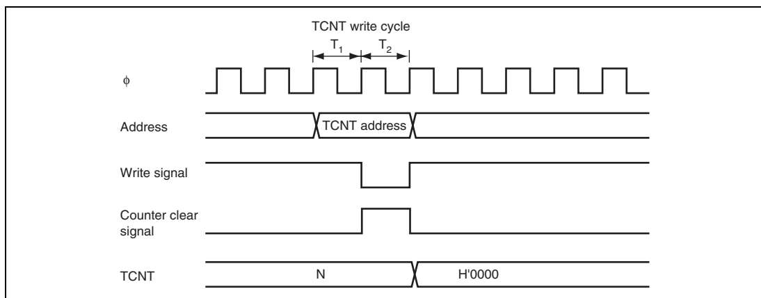
Figure 13.24 Contention between TCNT Write and Clear
