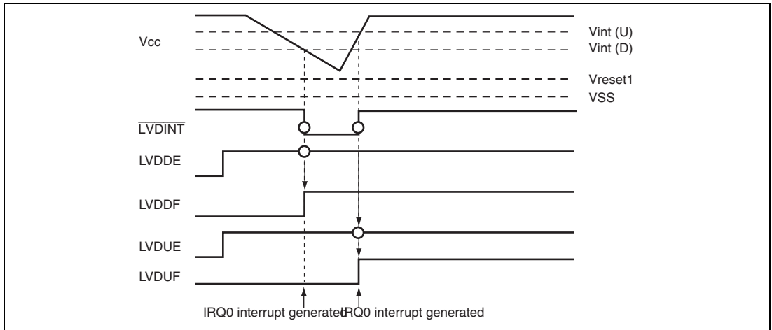
Figure 20.4 Operational Timing of LVDR Circuit
