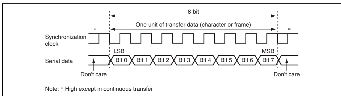
Figure 17.9 Data Format in Clocked Synchronous Communication
