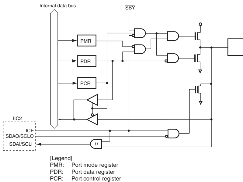
Figure B.12 Port 5 Block Diagram (P57, P56)
