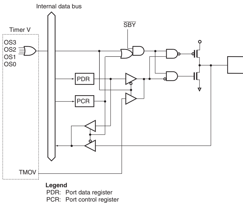
Figure B.14 Port 7 Block Diagram (P76)
