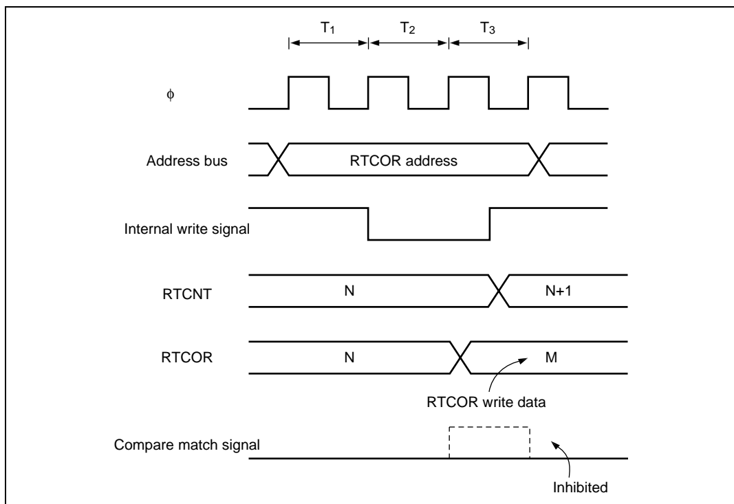
Figure 6.41 Contention between RTCOR Write and Compare Match
