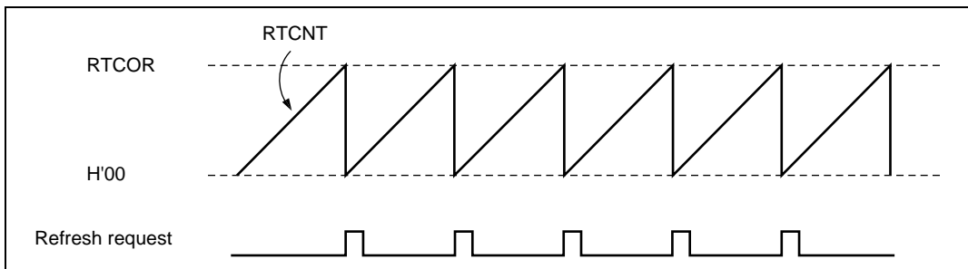
Figure 6.26 RTCNT Operation
