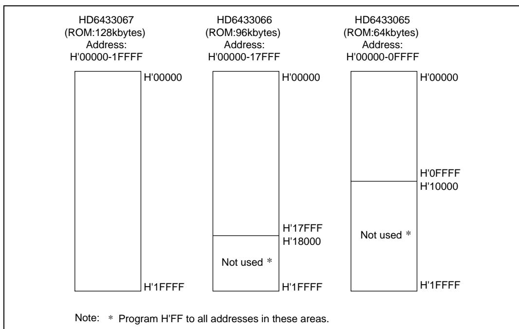
Figure 18.29 Mask ROM Addresses and Data
