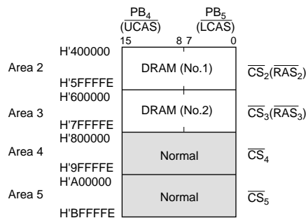
Figure 6.31 Interconnections and Address Map for 2-CAS 16-Mbit DRAMs with × 16-Bit Organization
