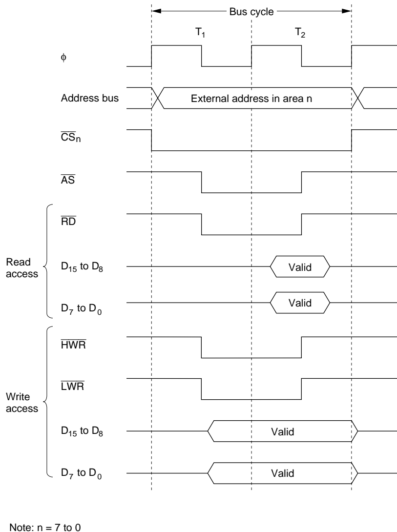
Figure 6.11 Bus Control Signal Timing for 16-Bit, Two-State-Access Area (3) (Word Access)
