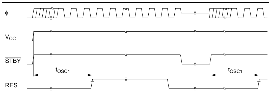
Figure 21.7 Oscillator Settling Timing
