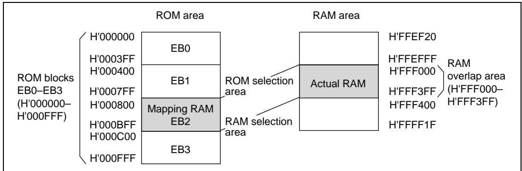
Figure 18.2 Example of ROM Area/RAM Area Overlap
