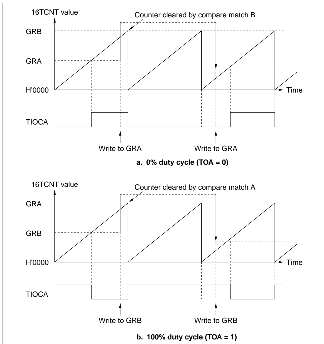
Figure 8.28 PWM Mode (Example 2)
