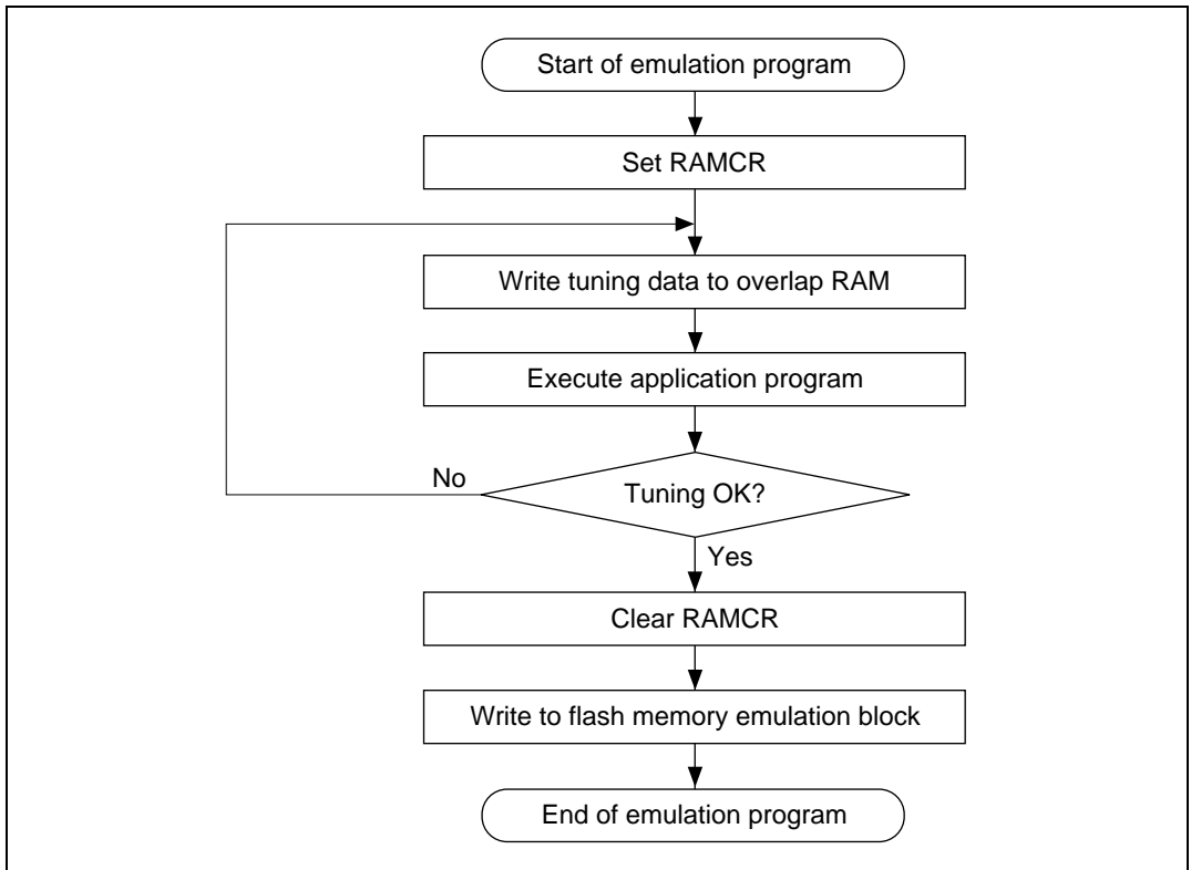
Figure 17.13 Flowchart of Flash Memory Emulation in RAM
