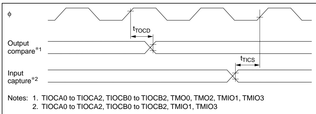
Figure 21.16 Timer Input/Output Timing
