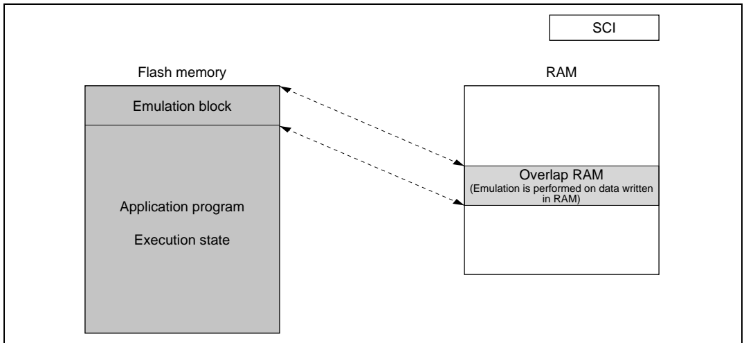
Figure 18.4 Reading Overlap RAM Data in User Mode/User Program Mode
