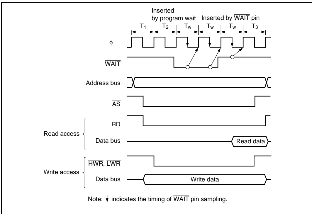
Figure 6.16 Example of Wait State Insertion Timing
