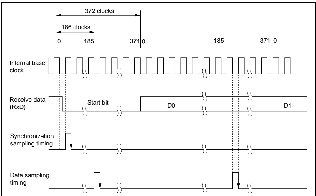
Figure 13.11 Receive Data Sampling Timing in Smart Card Interface Mode
