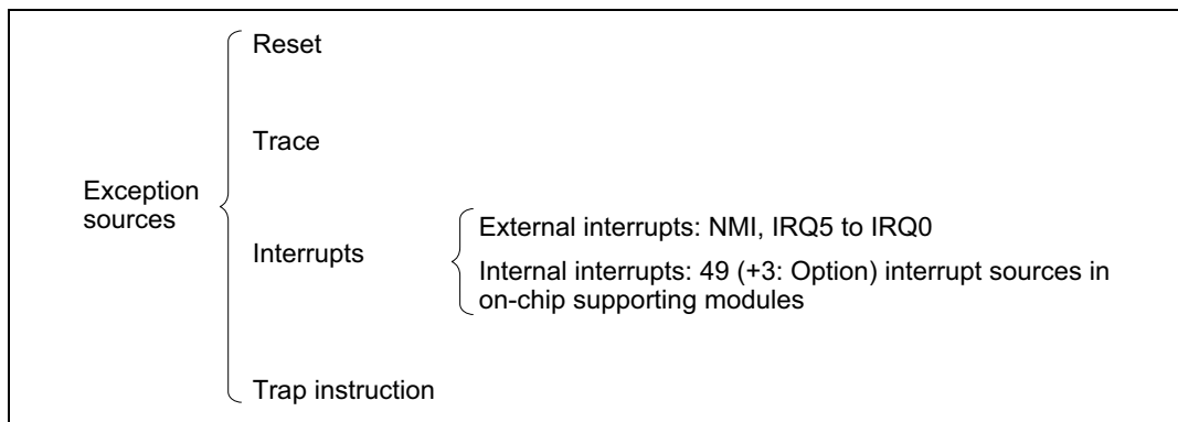
Figure 4-1 Exception Sources
