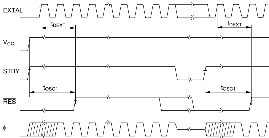
Figure 24-10 Oscillator Settling Timing
