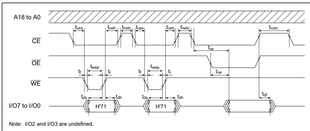
Figure 21A-24 Status Read Mode Timing Waveforms
