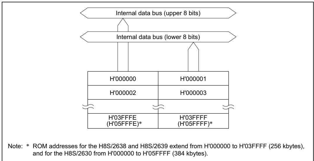
Figure 21B-1 Block Diagram of ROM 256 kbytes (384 kbytes)*
