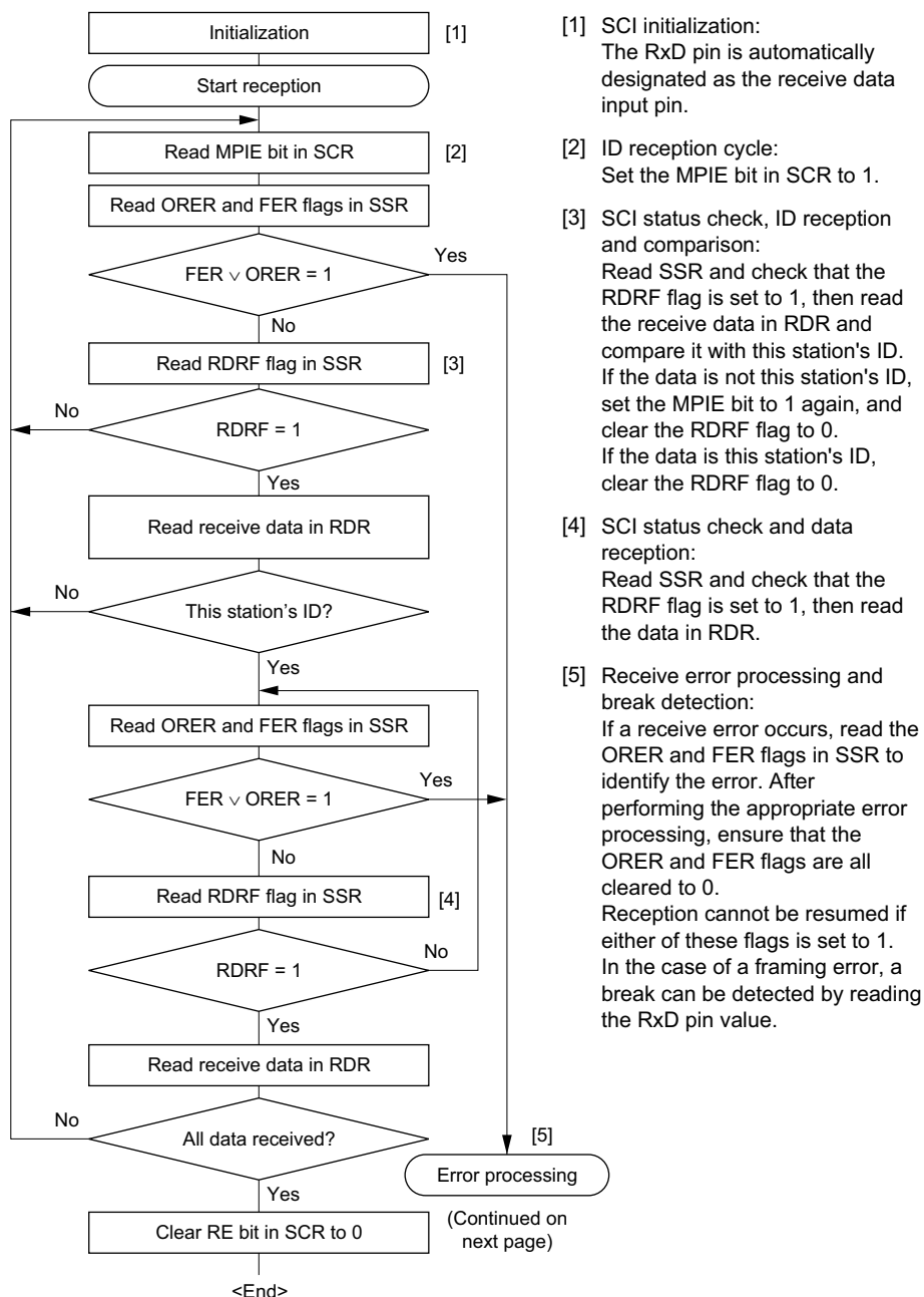
Figure 13-12 Sample Multiprocessor Serial Reception Flowchart
