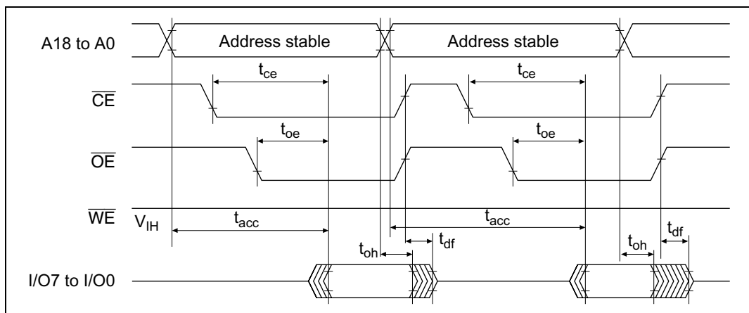
Figure 21B-21 \overline{\text{CE}} and \overline{\text{OE}} Clock System Read Timing Waveforms
