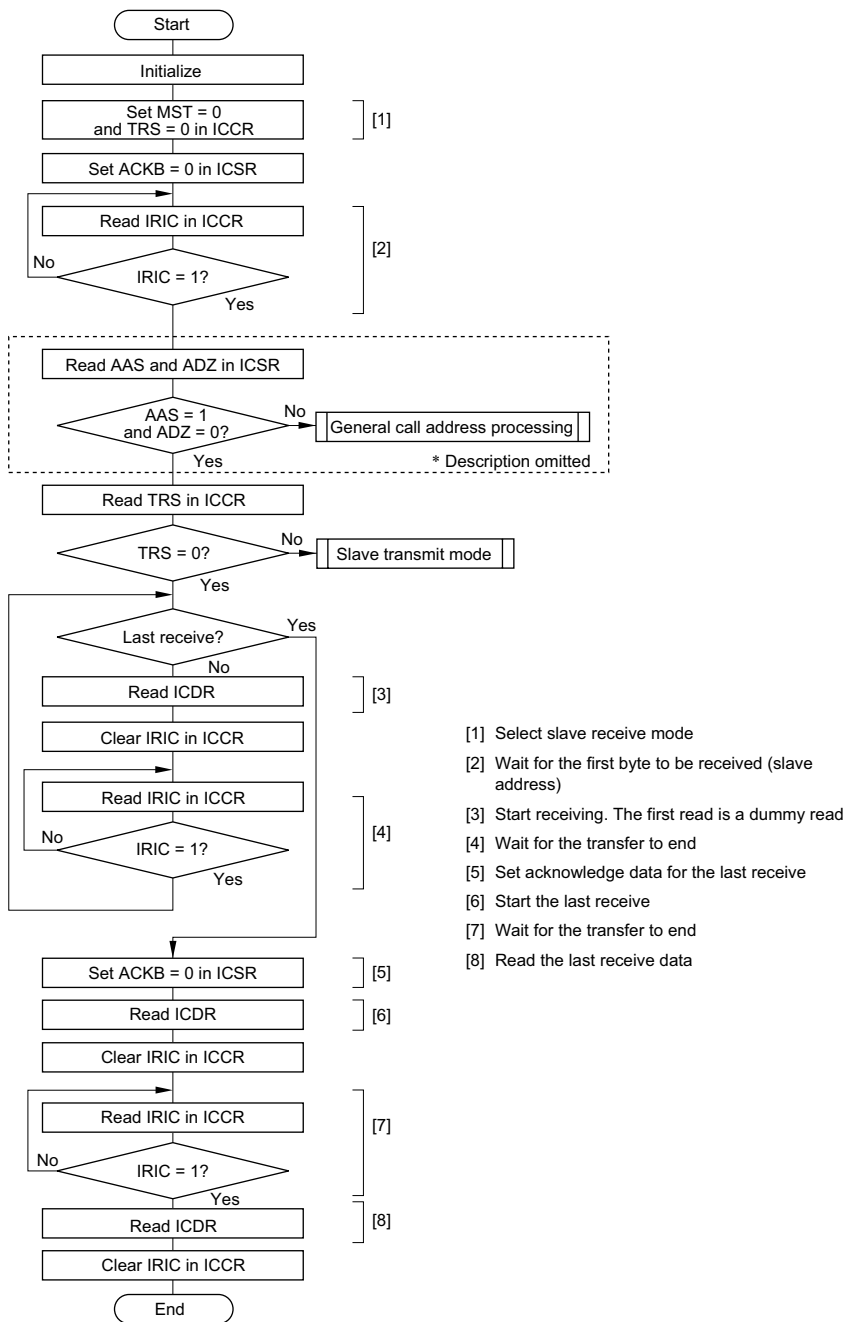
Figure 15-14 Flowchart for Slave Transmit Mode (Example)
