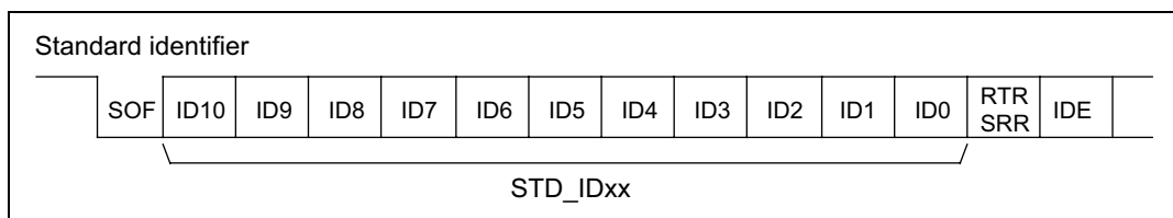
Figure 16-2 Standard identifier
