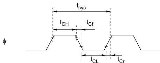
Figure 24-9 System Clock Timing
