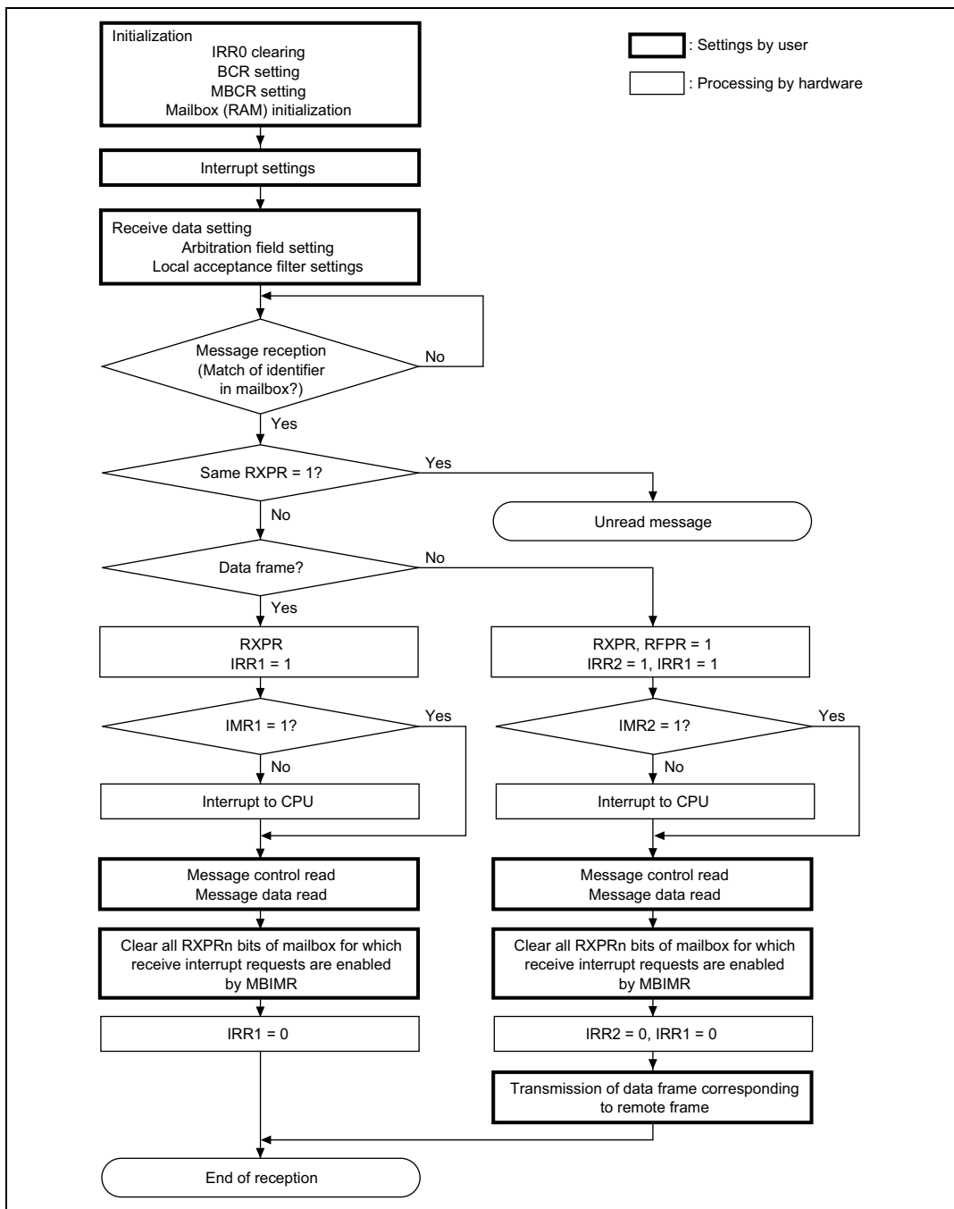
Figure 16-9 Reception Flowchart
