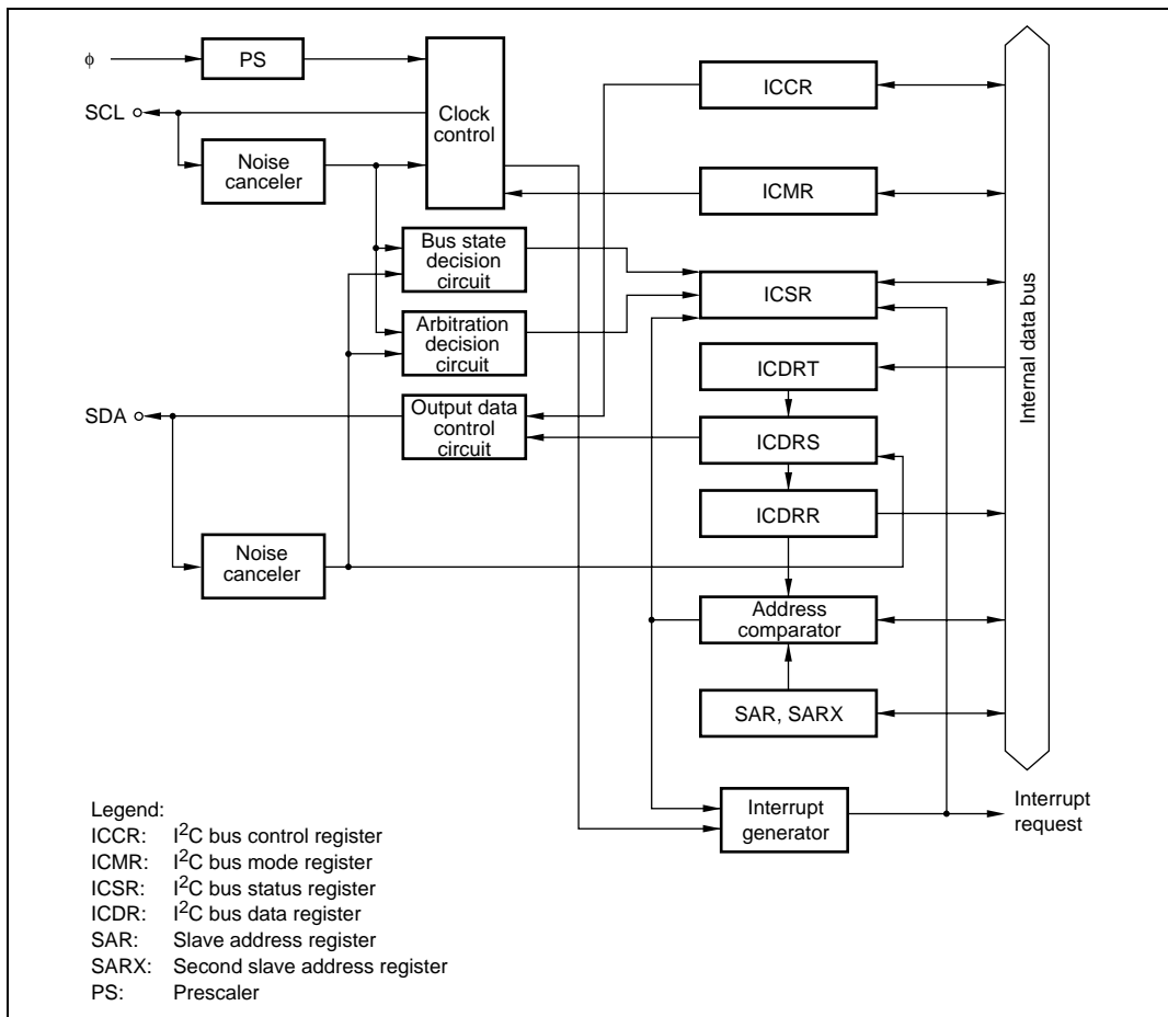
Figure 16.1 Block Diagram of I 2 C Bus Interface
