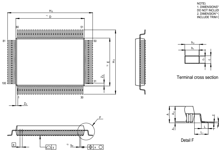
Figure C.3 FP-100A Package Dimensions
