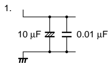
Figure 17.10 Example of Analog Input Protection Circuit
