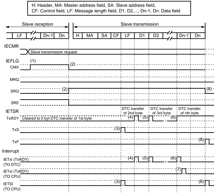
Figure 14.12 Slave Transmit Operation Timing
