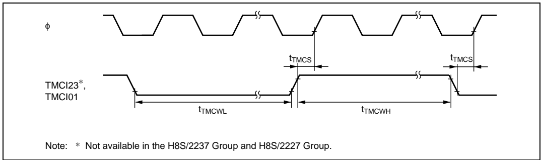
Figure 27.28 8-Bit Timer Clock Input Timing
