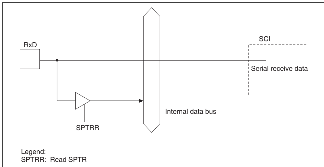
Figure 15.4 RxD Pin
