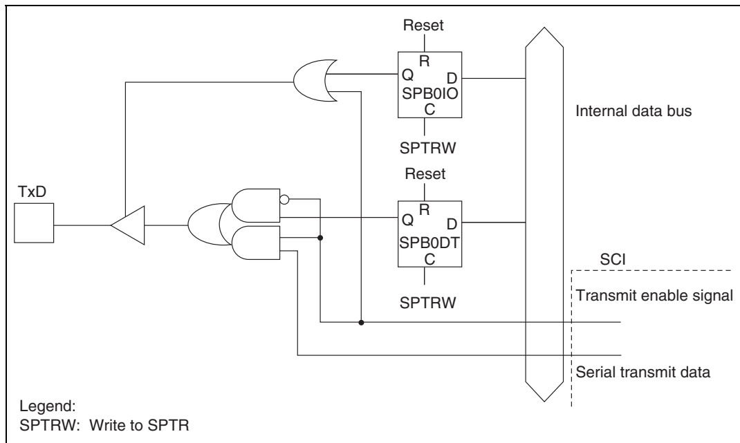
Figure 15.3 TxD Pin
