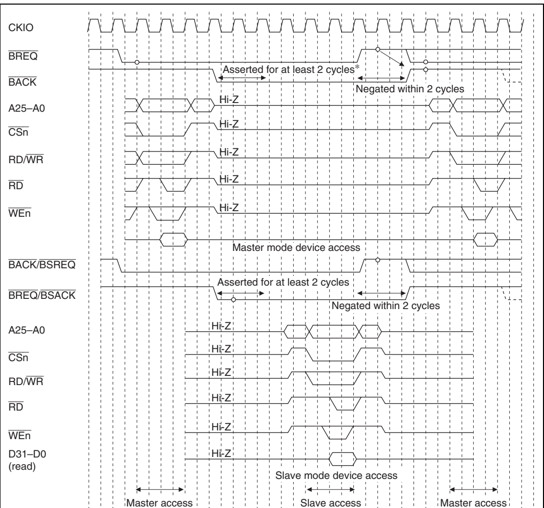
Figure 13.69 Arbitration Sequence
