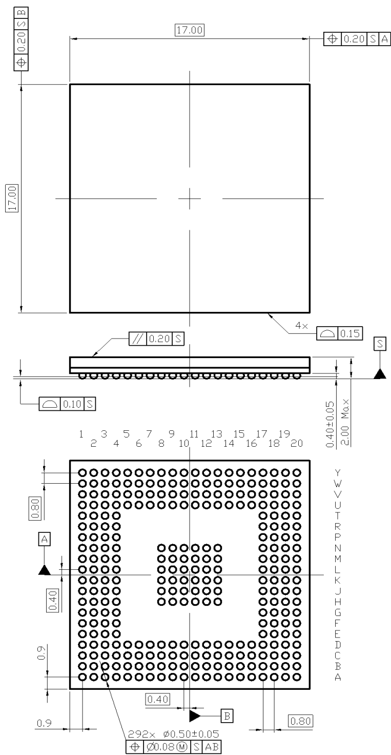
Appendix 3 17mm × 17mm (PRBG0292GA-A) Package dimension
