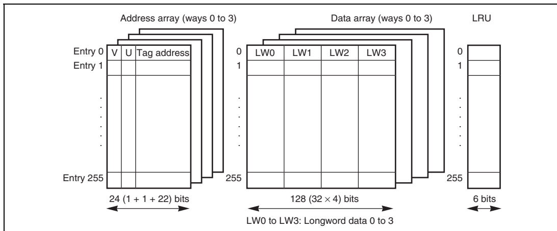
Figure 5.1 Cache Structure
