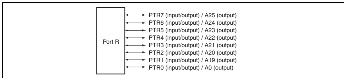
Figure 35.14 Port R
