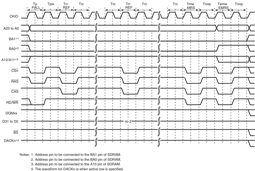
Figure 9.29 EMRS Command Issue Timing
