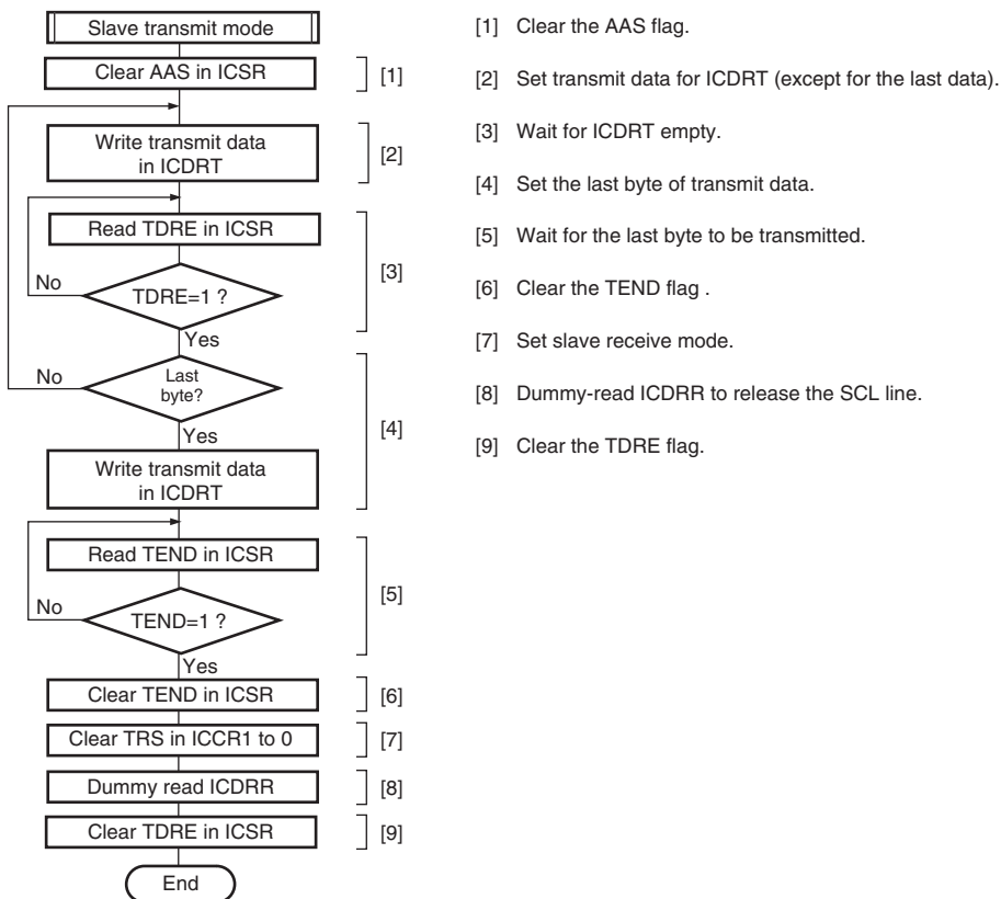
Figure 20.16 Sample Flowchart for Slave Transmit Mode
