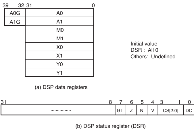
Figure 3.3 DSP Register Configuration
