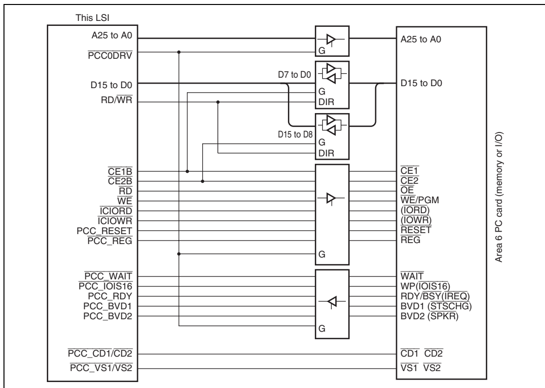
Figure 29.4 Interface
