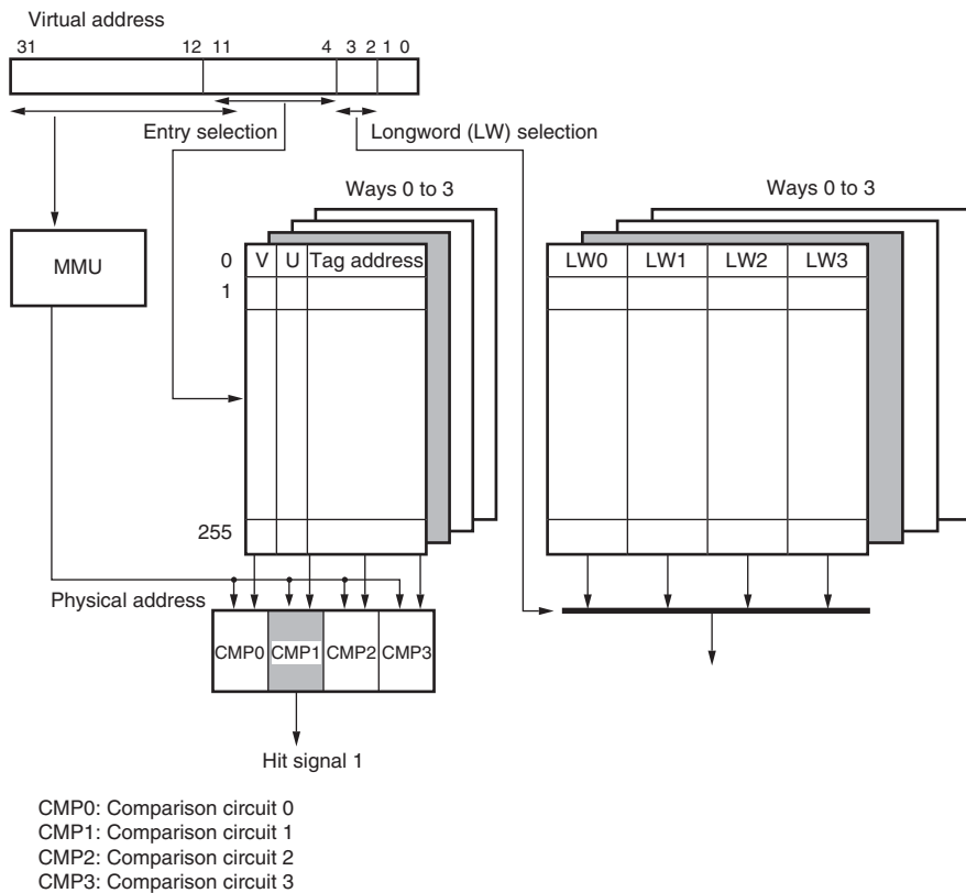
Figure 5.2 Cache Search Scheme
