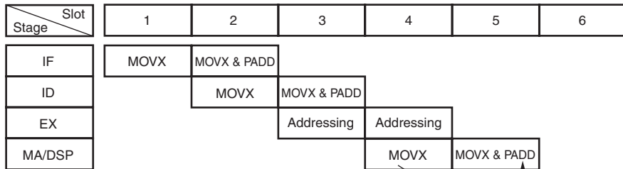
Figure 3.10 Operation Sequence Example
