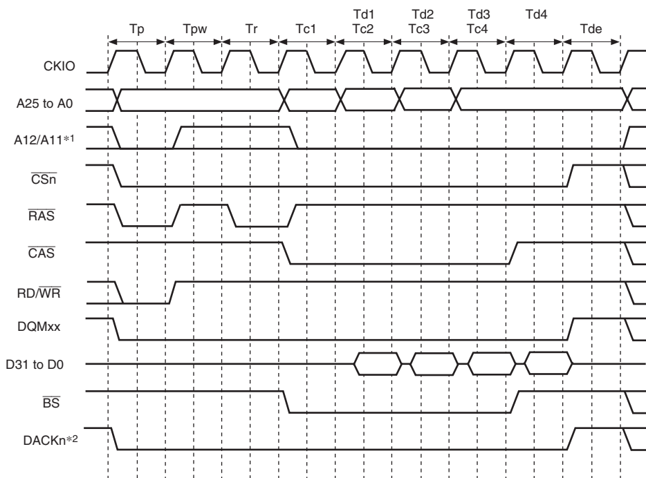
Figure 9.21 Burst Read Timing (Bank Active, Different Row Addresses)
