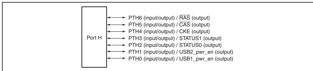
Figure 35.8 Port H
