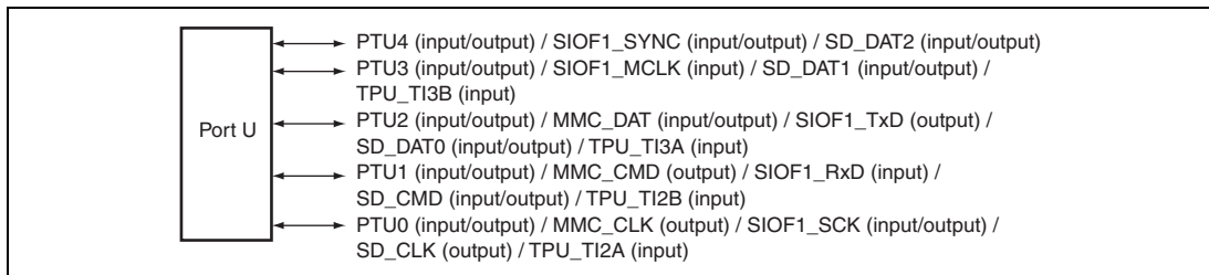
Figure 35.17 Port U
