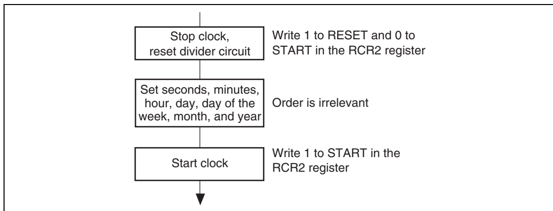
Figure 17.2 Setting Time
