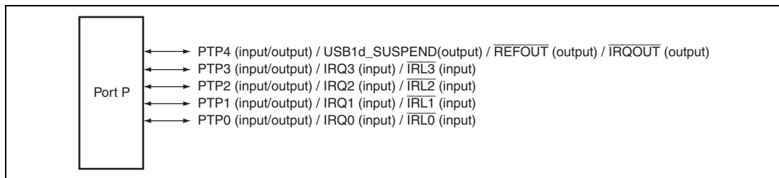
Figure 35.13 Port P
