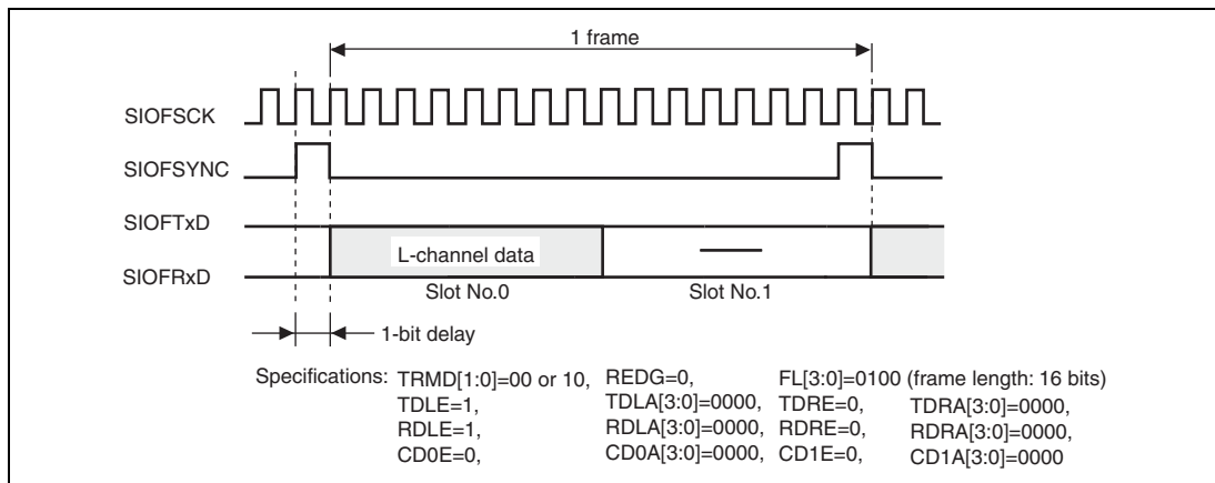
Figure 21.14 Transmit and Receive Timing (8-Bit Monaural Data (2))
