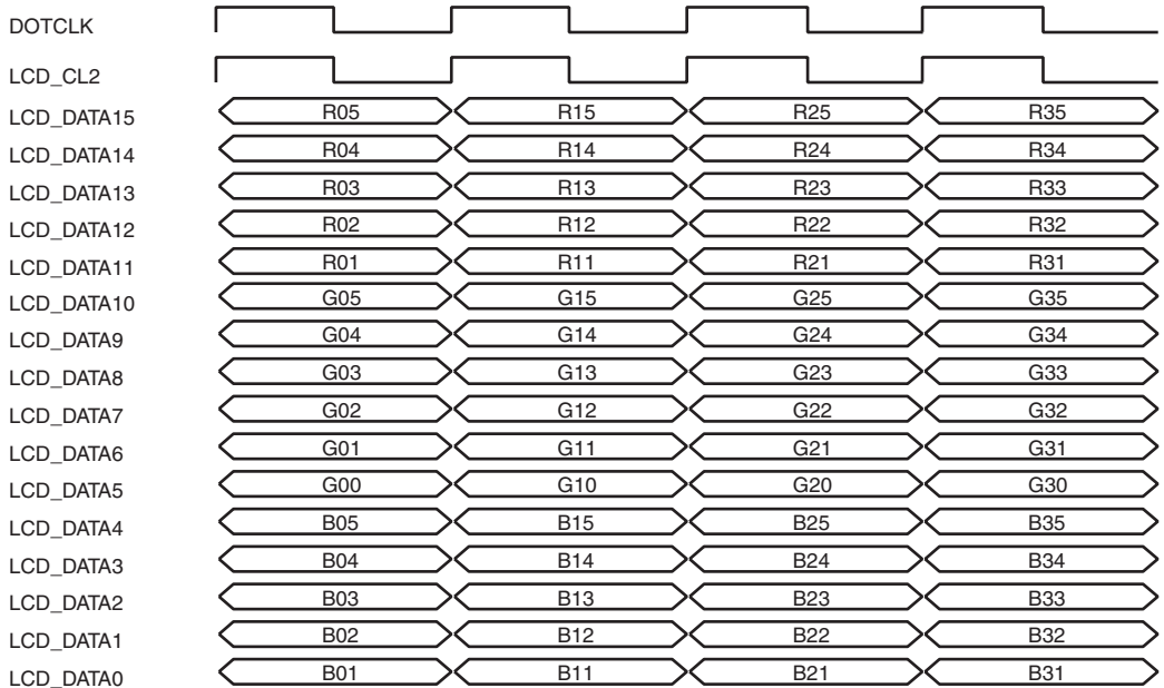
Figure 26.21 Clock and LCD Data Signal Example (TFT Color 16-Bit Data Bus Module)
