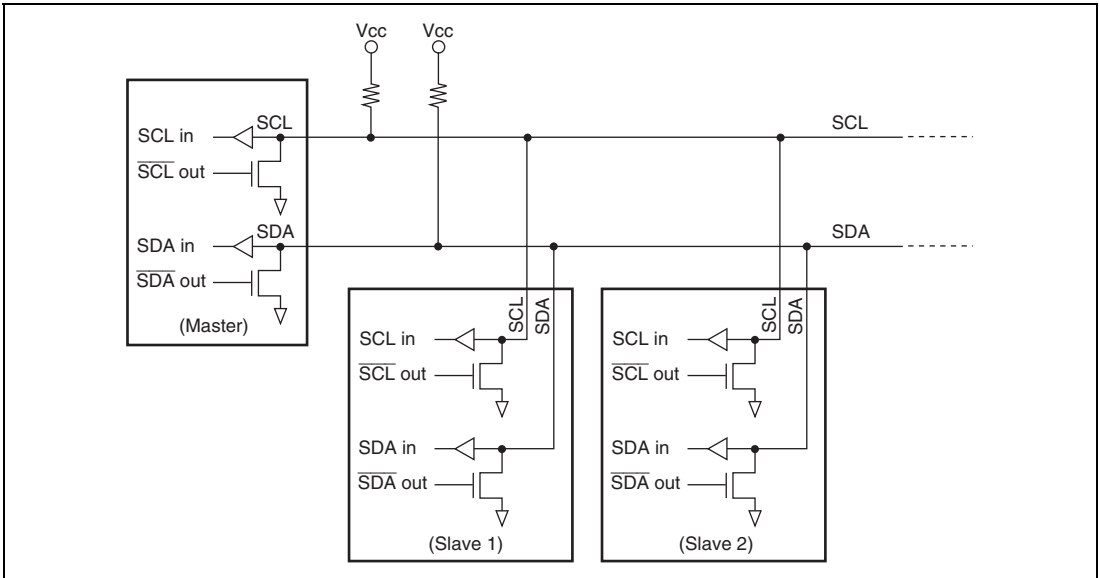
Figure 20.2 External Circuit Connections of I/O Pins
