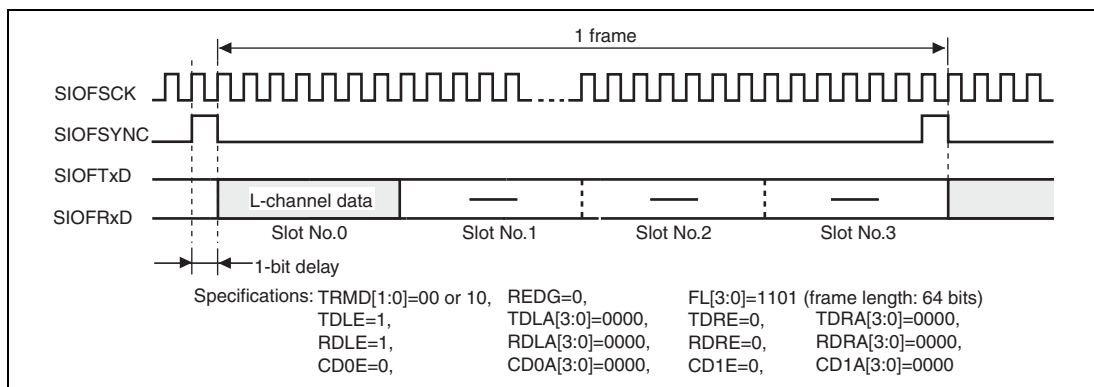
Figure 21.15 Transmit and Receive Timing (16-Bit Monaural Data (1))
