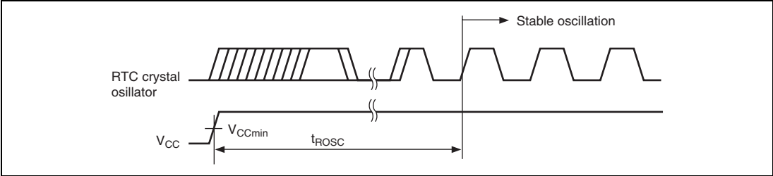
Figure 38.49 Oscillation Settling Time when RTC Crystal Oscillator is Turned On
