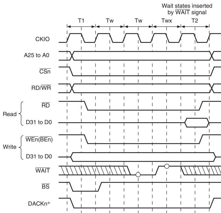
Figure 9.10 Wait State Timing for Normal Space Access (Wait State Insertion using \overline{\text{WAIT}} Signal)
