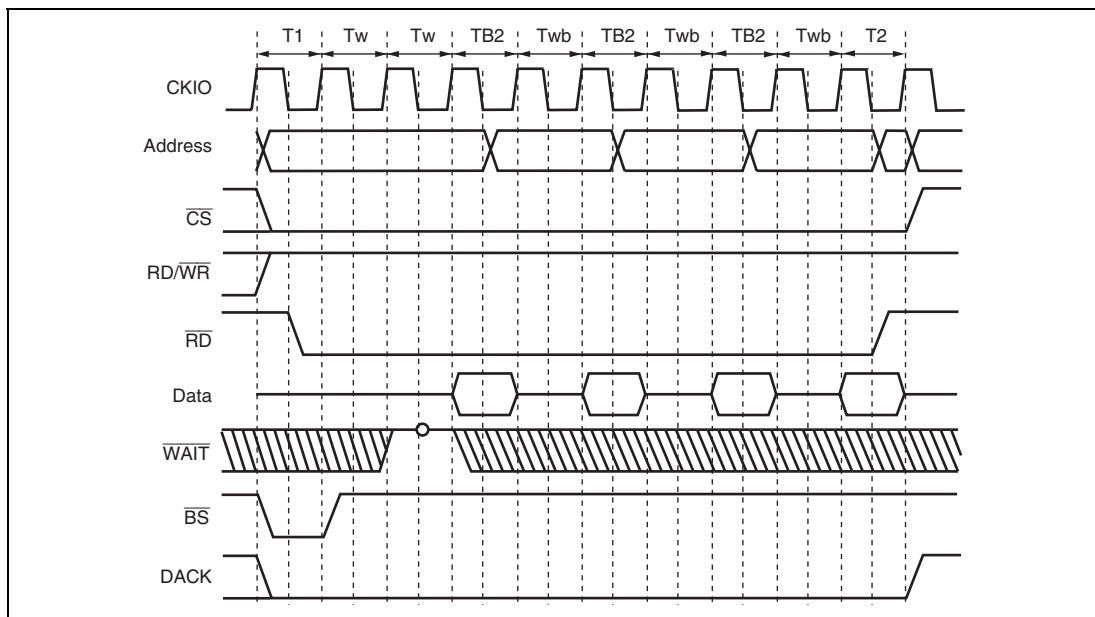
Figure 9.31 Burst ROM (Clock Asynchronous) Access (Bus Width = 32 Bits, 16-byte Transfer (Number of Bursts = 4), Access Wait for First Time = 2, Access Wait for 2nd Time and after = 1)
