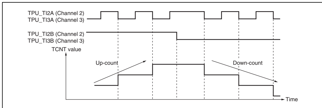
Figure 15.16 Example of Phase Counting Mode 2 Operation
