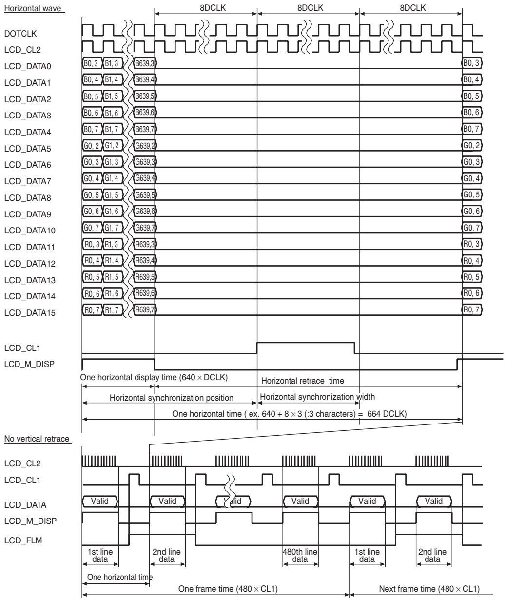
Figure 26.23 Clock and LCD Data Signal Example (16-Bit Interface Color 640 × 480)
