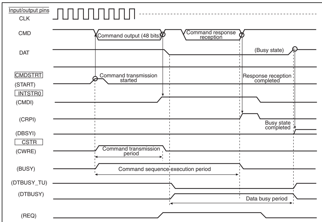
Figure 31.5 Example of Command Sequence for Commands without Data Transfer (with Data Busy State)
