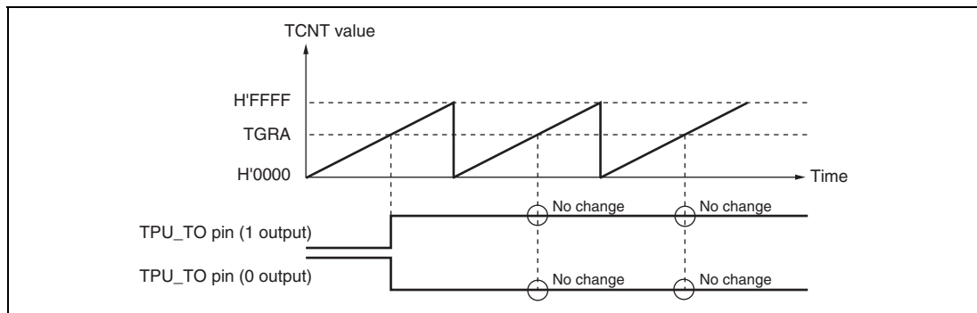
Figure 15.6 Example of 0 Output/1 Output Operation
