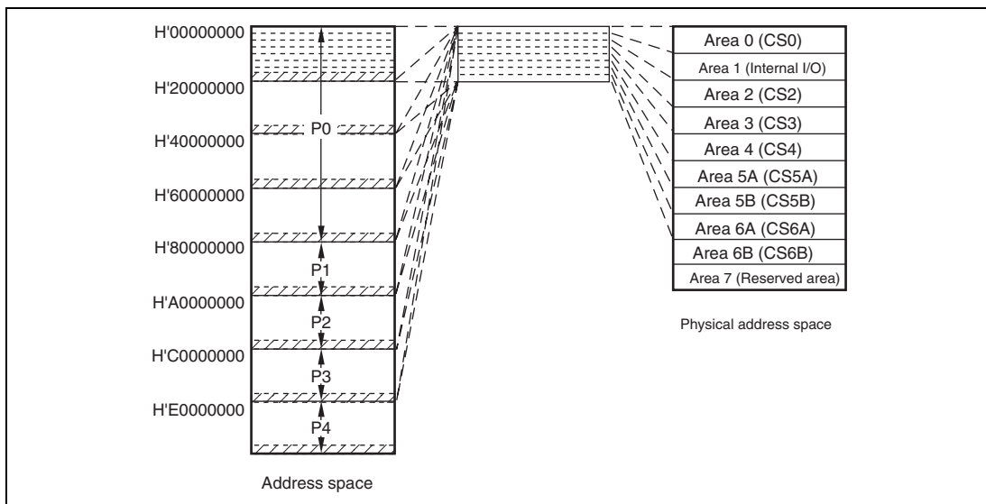
Figure 9.2 Address Space
