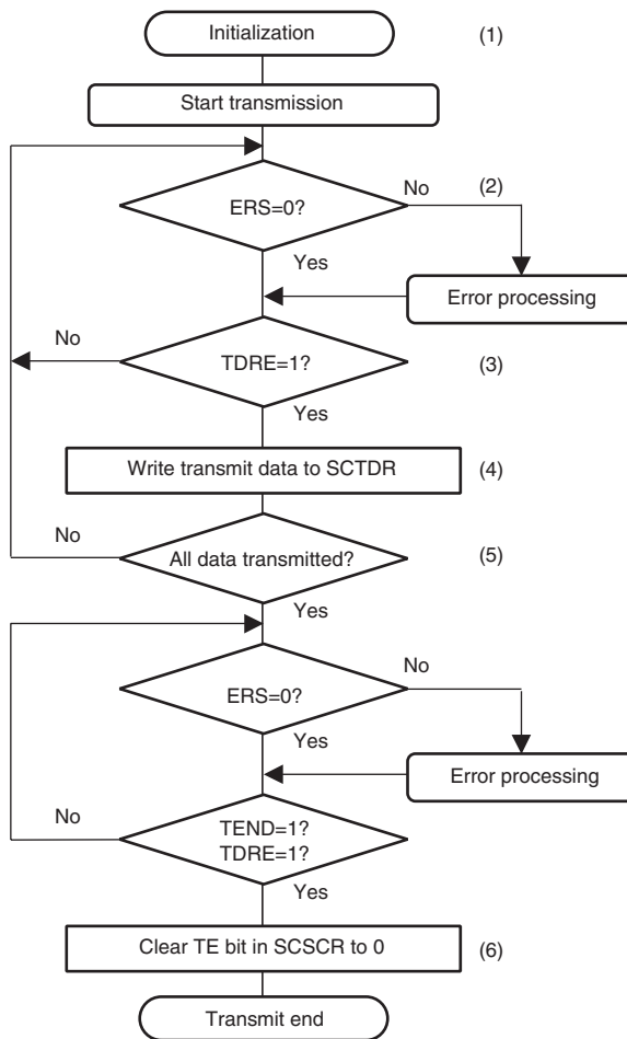
Figure 30.5 Example of Transmit Processing
