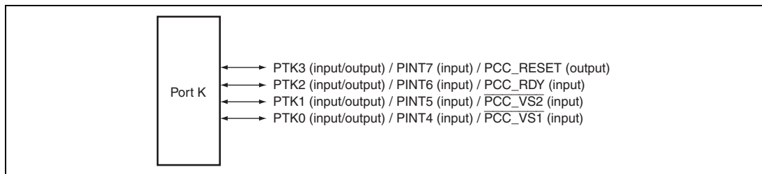
Figure 35.10 Port K
