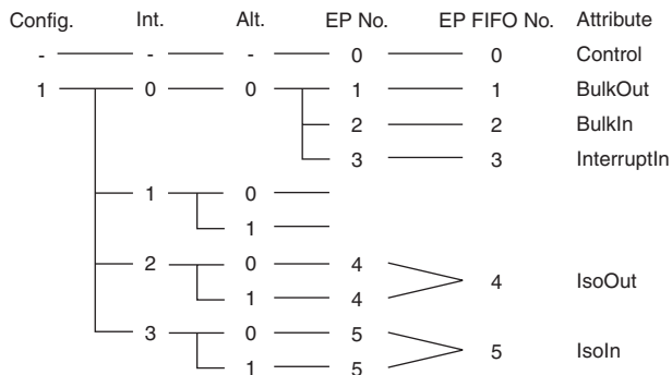
Figure 25.2 Example of Endpoint Configuration
