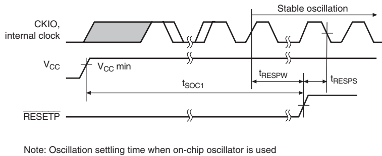
Figure 38.4 Power-On Oscillation Settling Time
