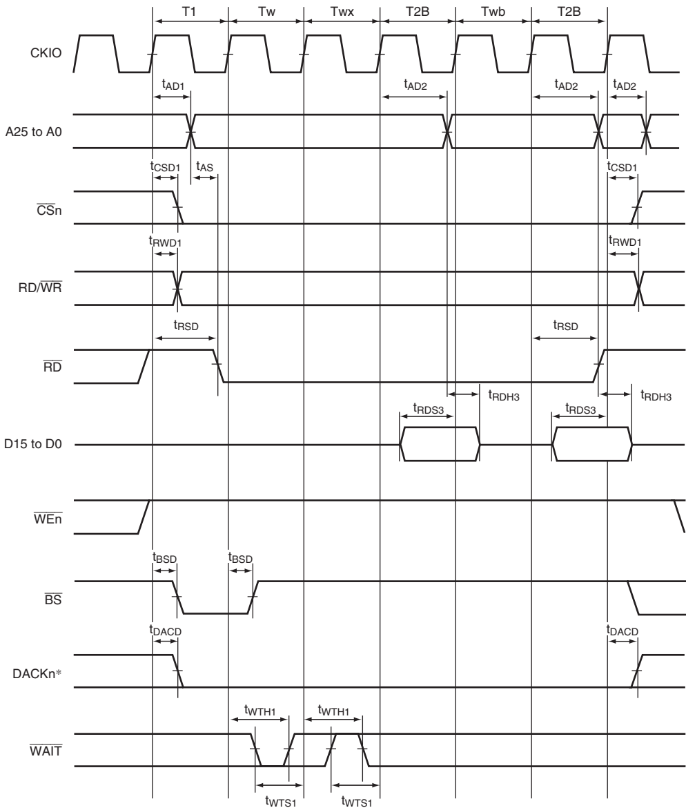
Figure 38.19 Read Bus Cycle of Burst ROM (Software Wait 1, External Wait 1 Input, Burst Wait 1, Number of Burst 2)
