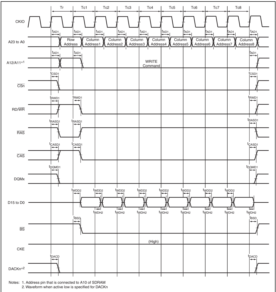
Figure 38.31 Burst Write Bus Cycle of SDRAM (Single Write x 8) (Bank Active Mode: ACTV + WRIT Command, TRCD = 1 Cycle)
