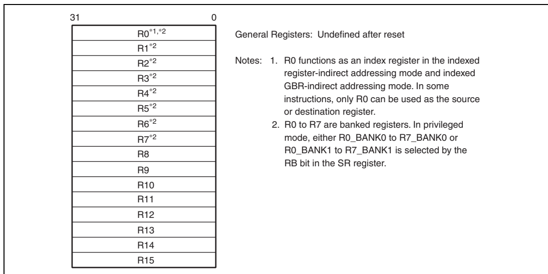
Figure 2.4 General Registers
