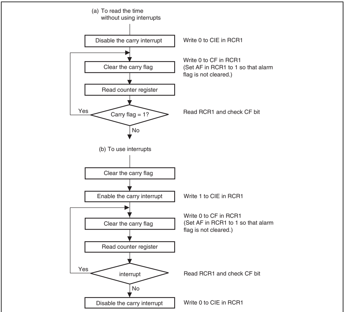
Figure 17.3 Reading Time
