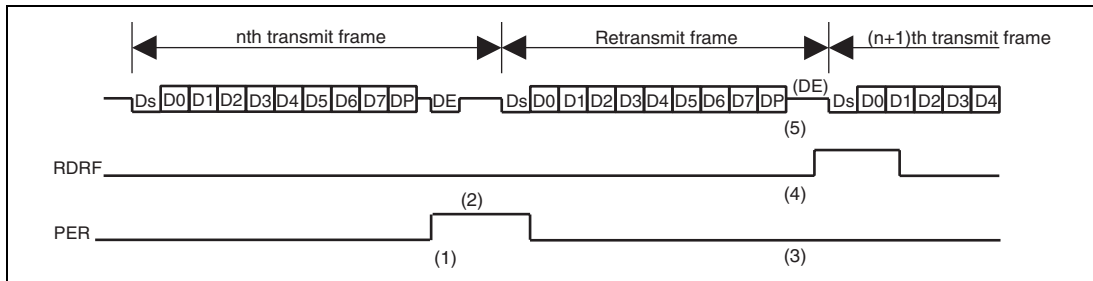
Figure 30.2 Retransmission when Smart Card Interface is in Receive Mode
