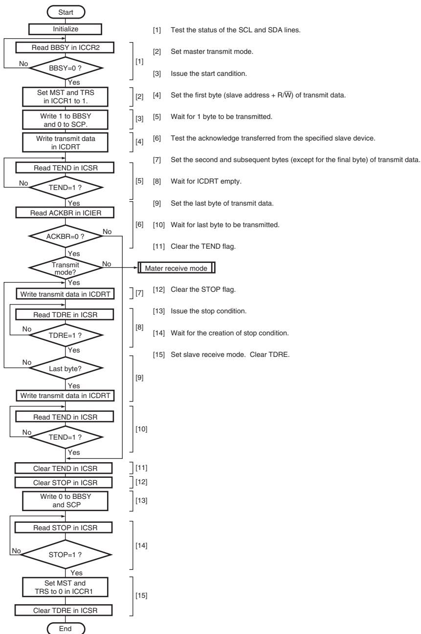
Figure 20.14 Sample Flowchart for Master Transmit Mode
