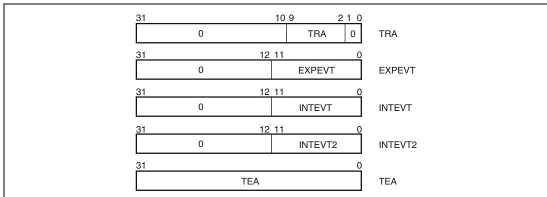
Figure 7.1 Register Bit Configuration
