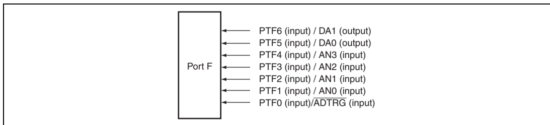
Figure 35.6 Port F
