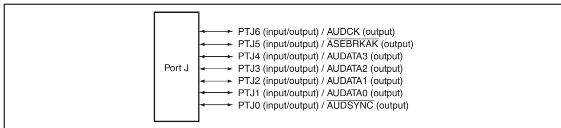
Figure 35.9 Port J
