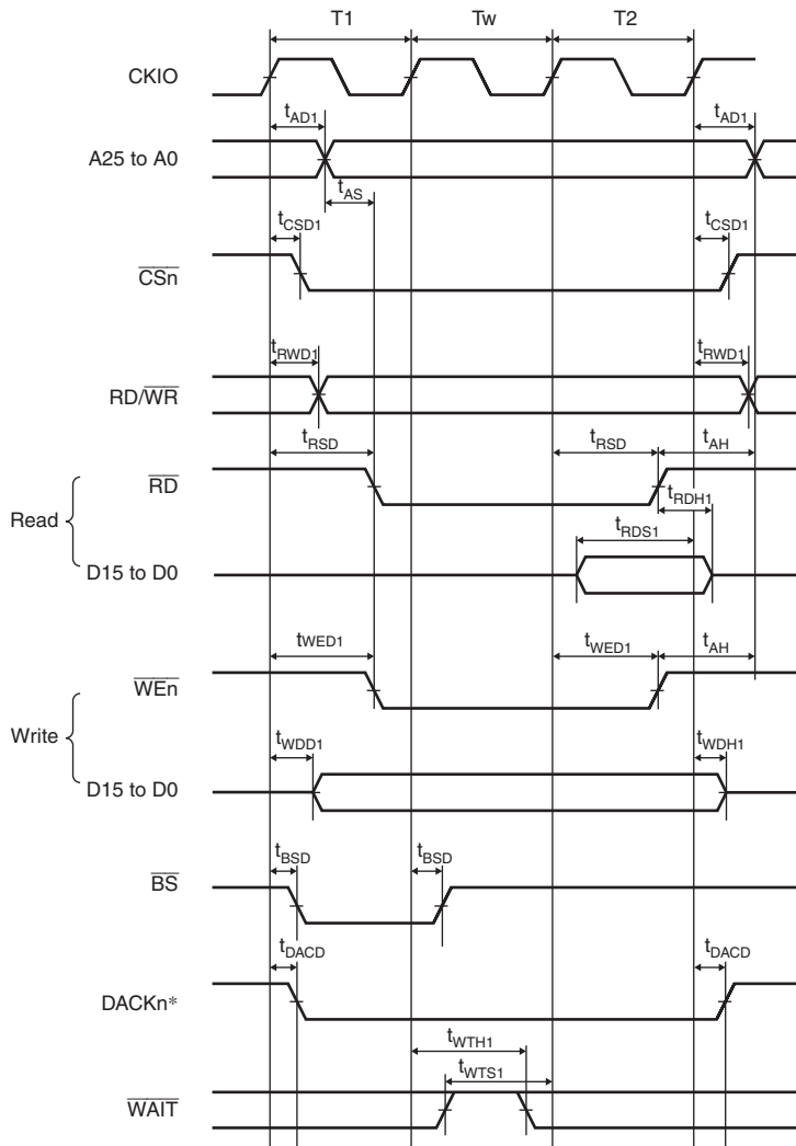
Figure 38.13 Basic Bus Cycle in Normal Space (Software Wait 1)
