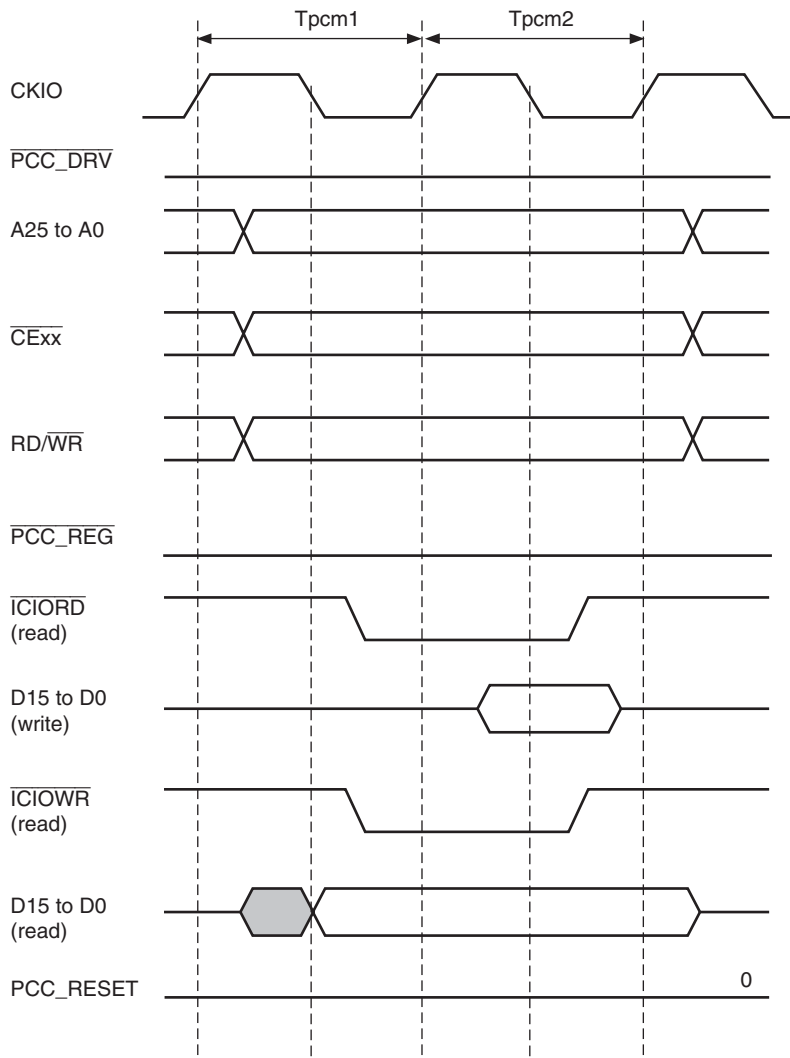
Figure 29.7 PCMCIA I/O Card Interface Basic Timing
