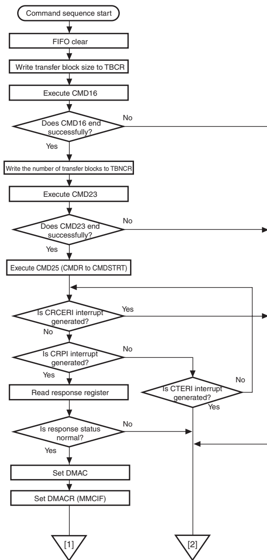
Figure 31.30 Operational Flowchart for Write Sequence (Pre-defined Multiblock Transfer) (1)
