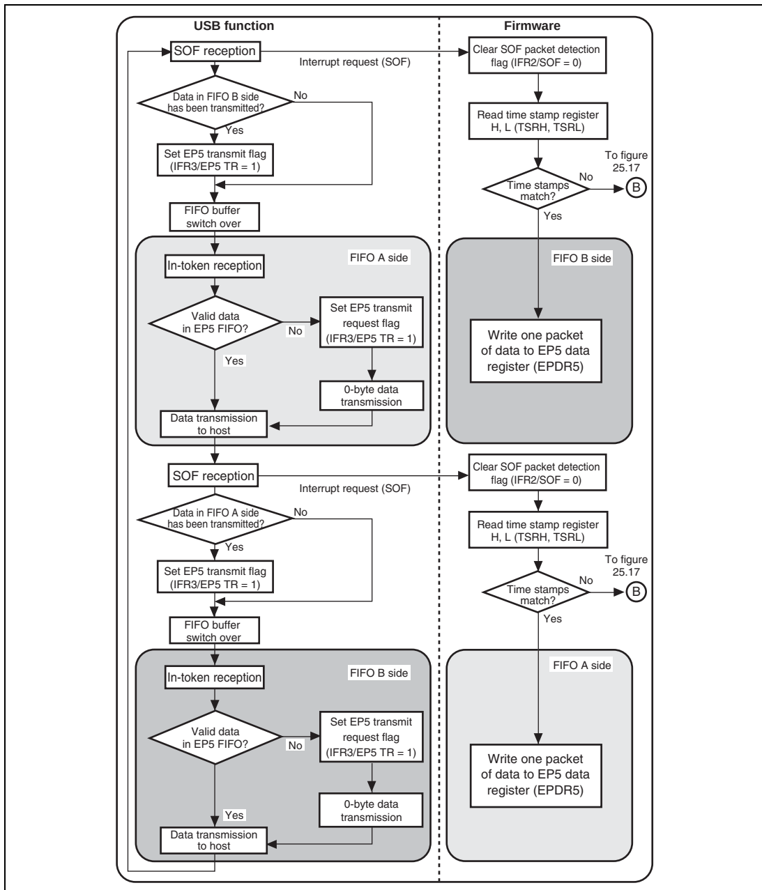
Figure 25.16 EP5 Isochronous-In Transfer Operation (SOF is Normal)
