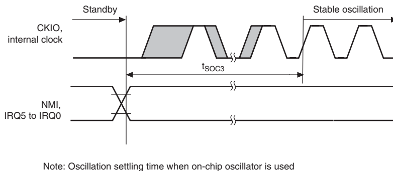
Figure 38.6 Oscillation Settling Time on Return from Standby (Return by NMI or IRQ)
