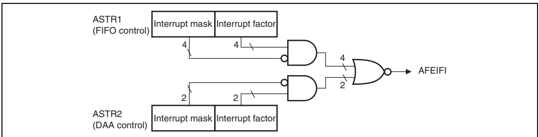
Figure 22.4 Interrupt Generator
