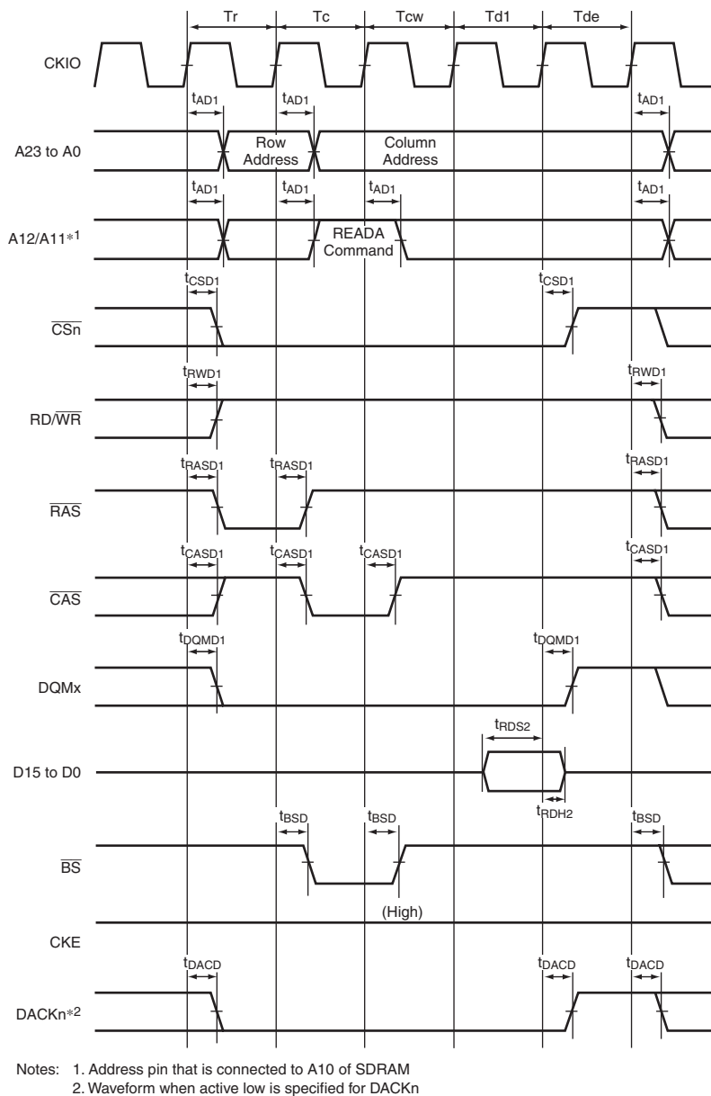
Figure 38.20 Single Read Bus Cycle of SDRAM (Auto Precharge Mode, CAS Latency 2, TRCD = 1 Cycle, TRP = 1 Cycle)
