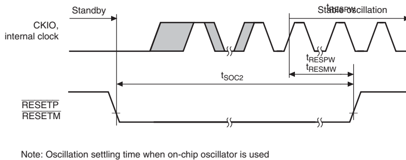
Figure 38.5 Oscillation Settling Time on Return from Standby (Return by Reset)
