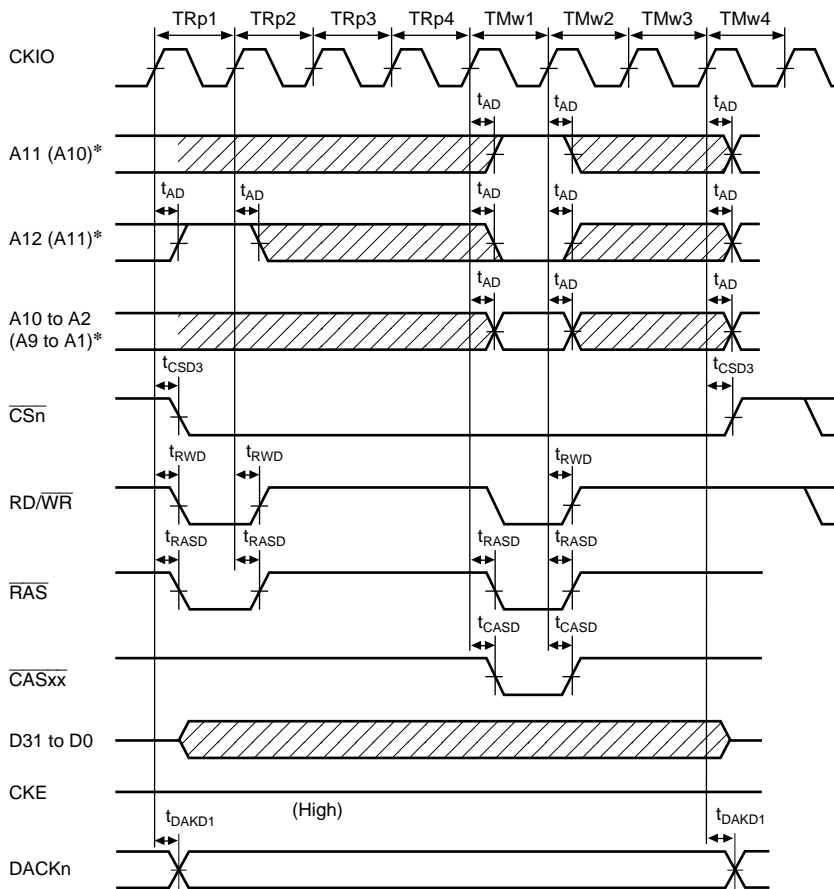
Figure 24.39 Synchronous DRAM Mode Register Write Cycle
