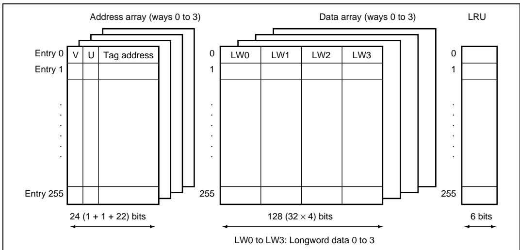
Figure 5.1 Cache Structure
