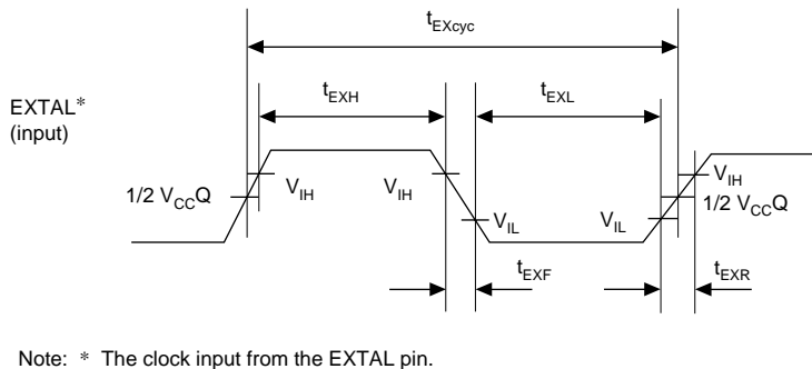
Figure 24.1 EXTAL Clock Input Timing
