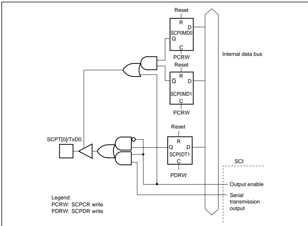
Figure 14.3 SCPT[0]/TxD0 Pin
