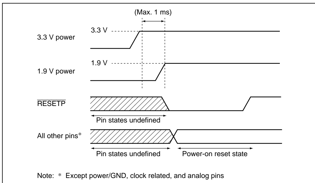
Power-On Sequence
