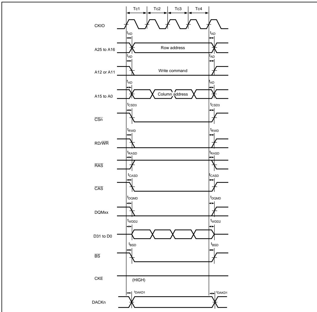
Figure 24.34 Synchronous DRAM Burst Write Bus Cycle (RAS Down, Same Row Address)
