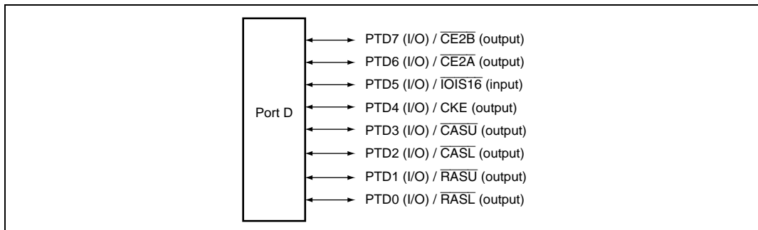
Figure 18.4 Port D
