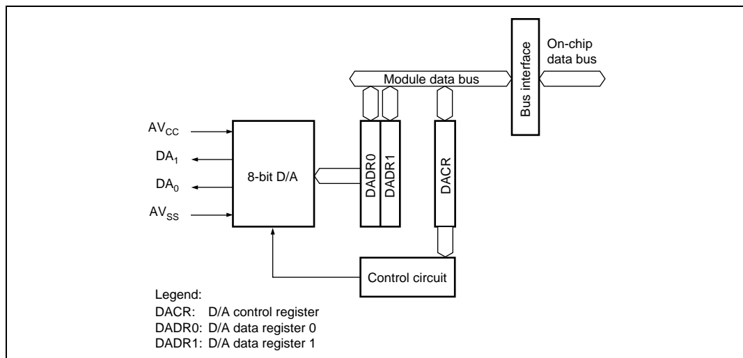
Figure 20.1 D/A Converter Block Diagram
