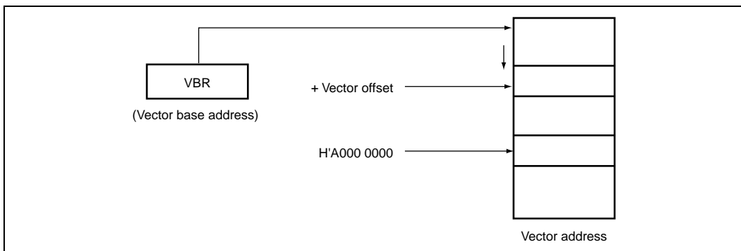
Figure 4.1 Vector Addresses
