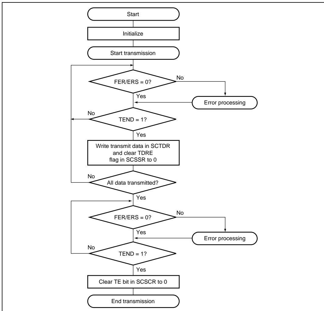
Figure 15.6 Transmission Flowchart
