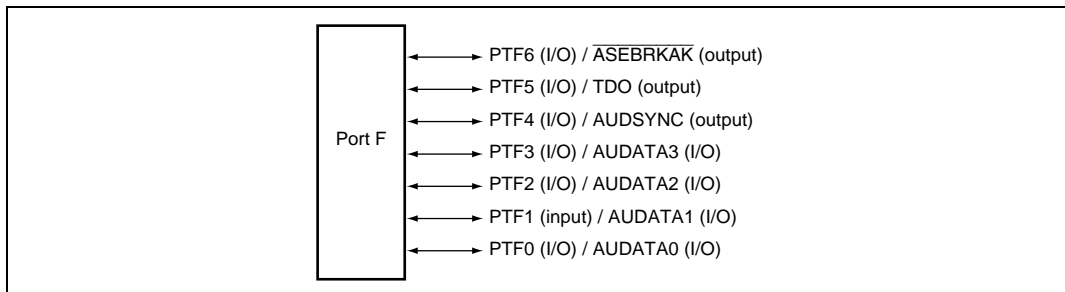
Figure 18.6 Port F
