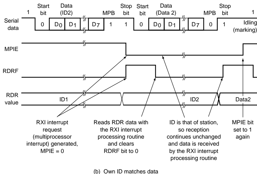
Figure 14.16 Example of SCI Receive Operation
