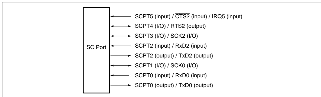
Figure 18.10 SC Port
