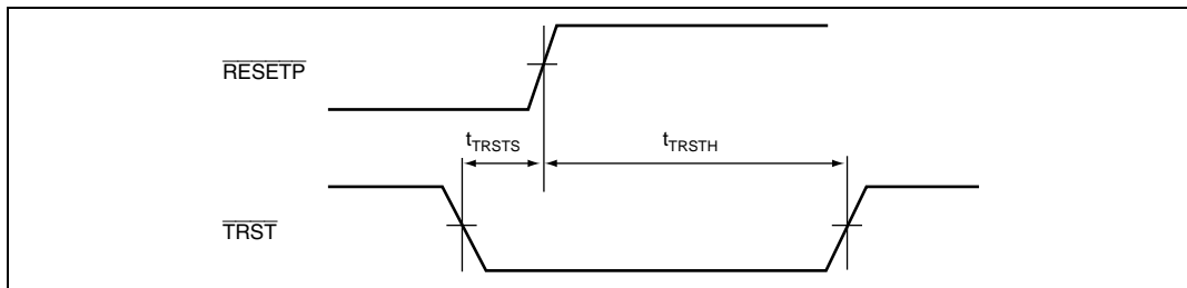
Figure 24.56 TRST Input Timing (Reset Hold)
