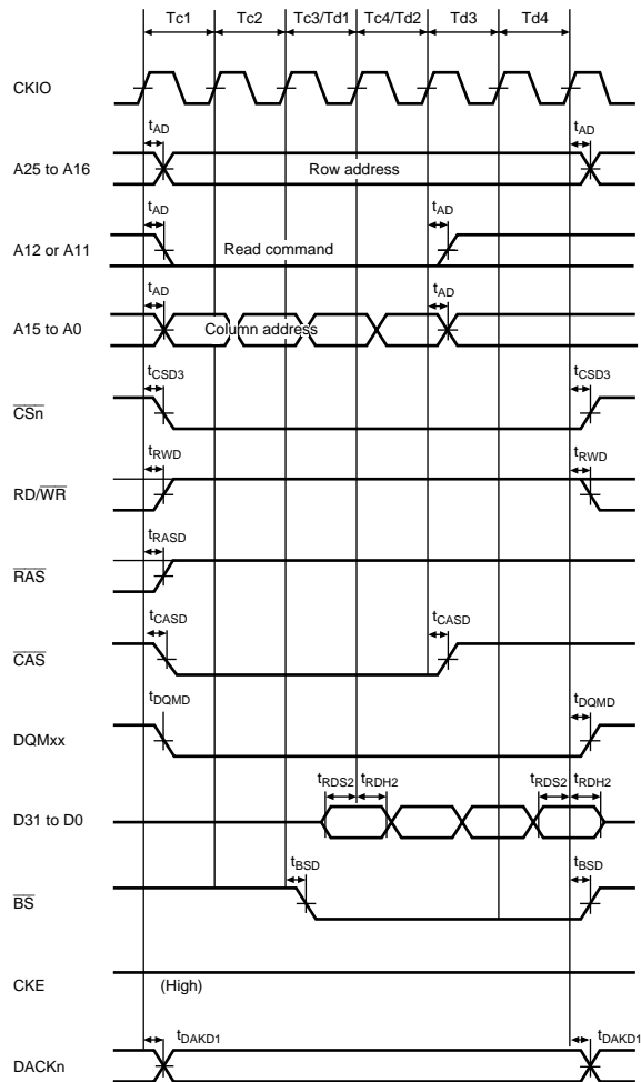
Figure 24.31 Synchronous DRAM Burst Read Bus Cycle (RAS Down, Same Row Address, CAS Latency = 2)
