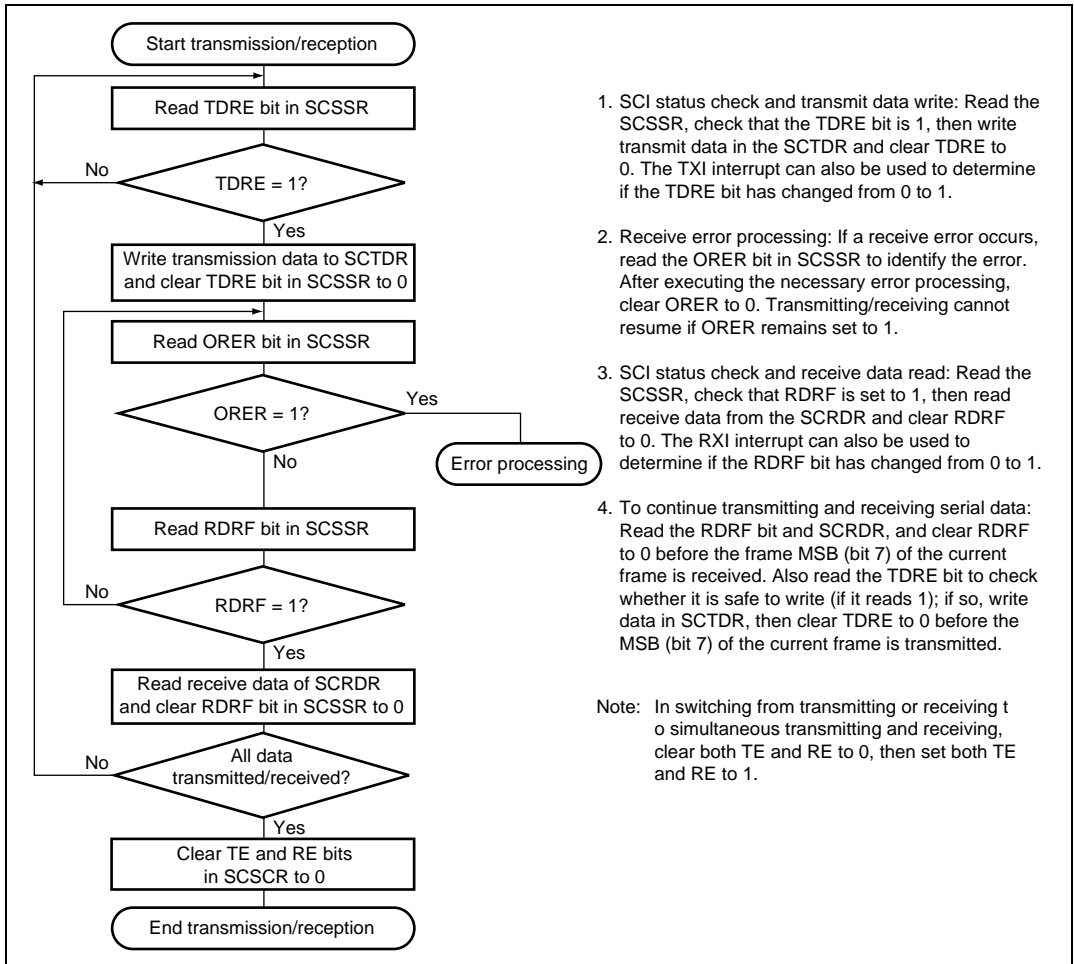
Figure 14.23 Sample Flowchart for Serial Data Transmitting/Receiving
