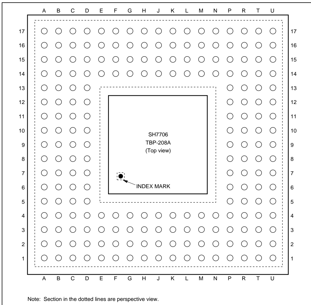
Figure 1.3 Pin Assignment (TBP-208A)
