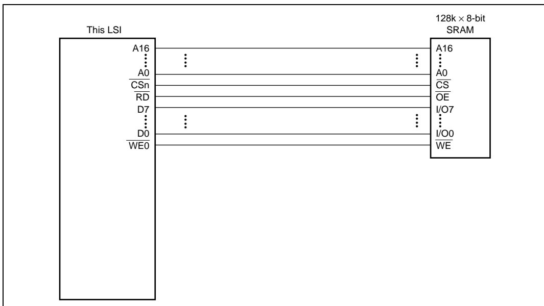
Figure 8.8 Example of 8-Bit Data-Width Static RAM Connection
