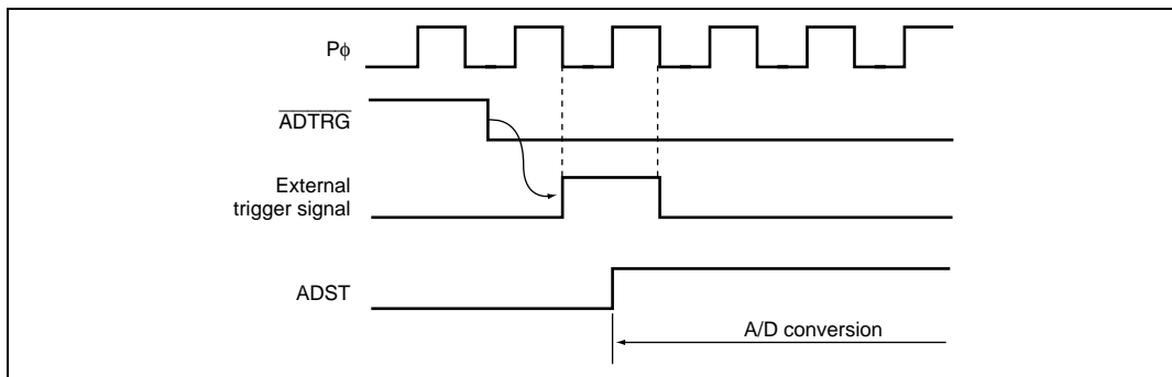
Figure 19.9 External Trigger Input Timing
