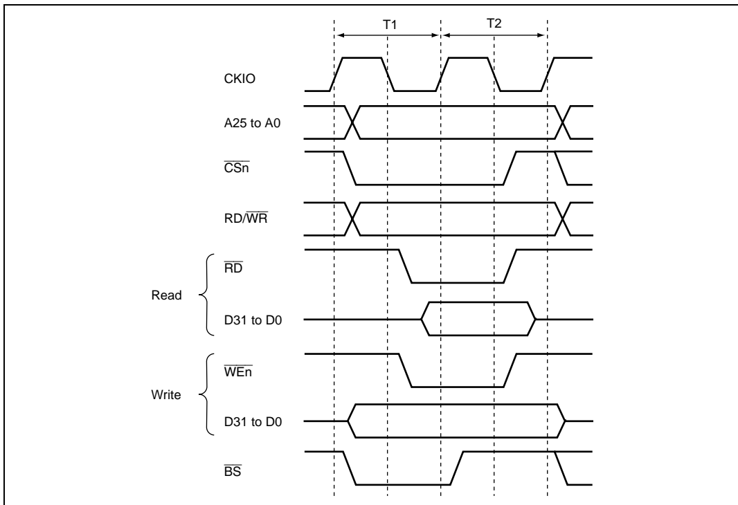
Figure 8.5 Basic Timing of Basic Interface
