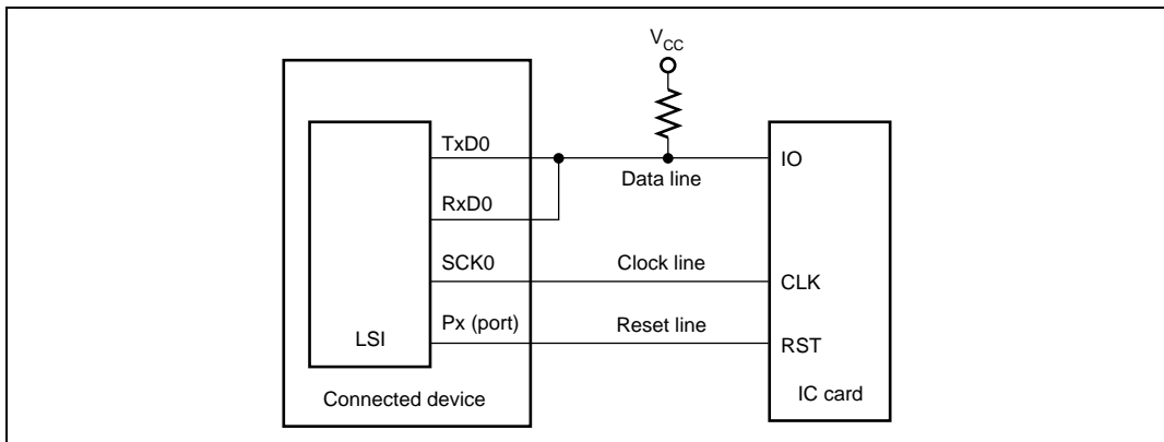
Figure 15.2 Pin Connection Diagram for the Smart Card Interface
