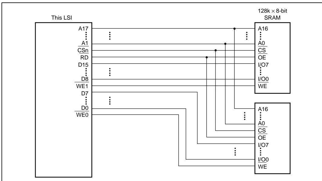
Figure 8.7 Example of 16-Bit Data-Width Static RAM Connection
