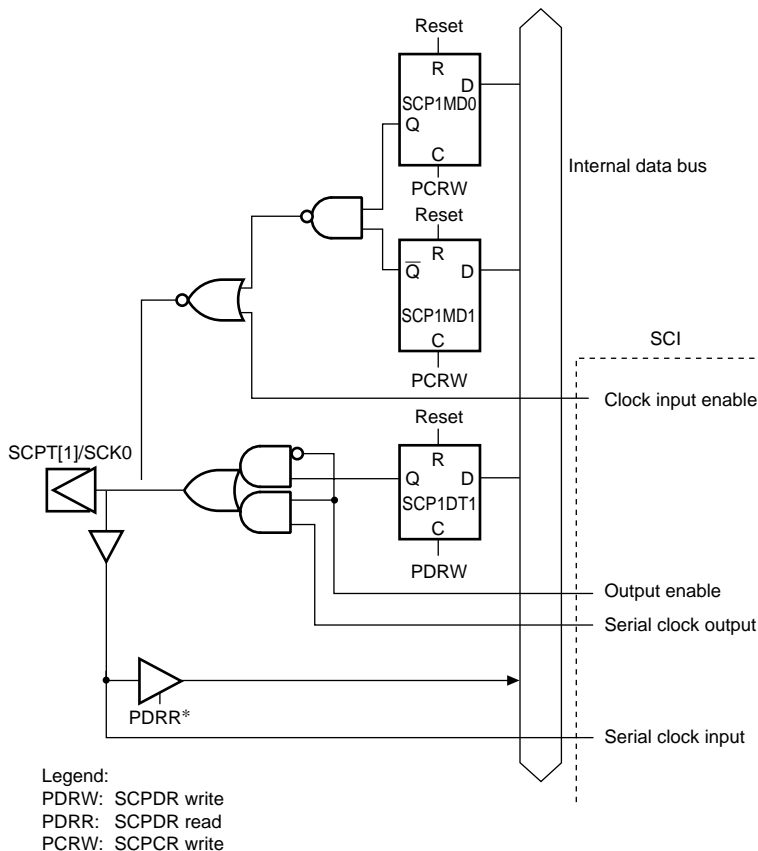
Figure 14.2 SCPT[1]/SCK0 Pin
