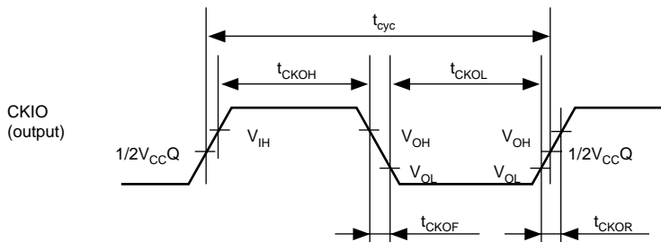
Figure 24.3 CKIO Clock Output Timing
