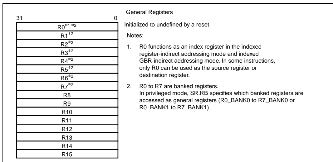
Figure 2.2 General Registers
