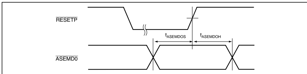
Figure 24.58 \overline{\text{ASEMD0}} Input Timing
