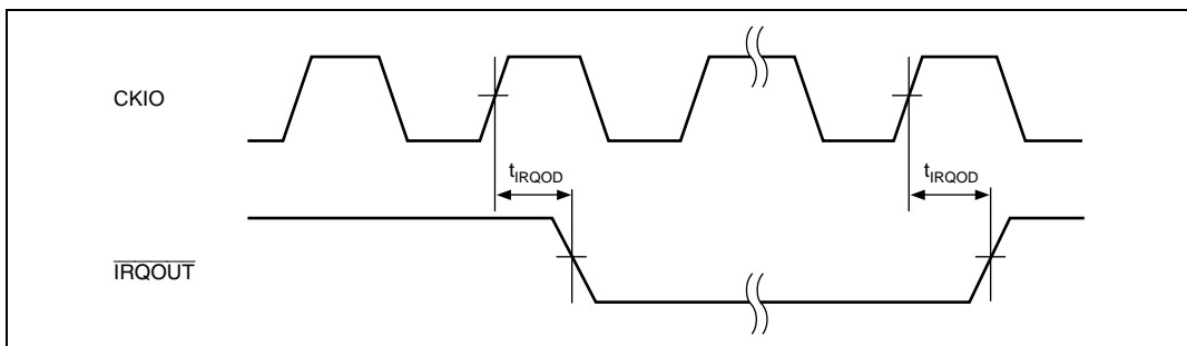
Figure 24.13 \overline{IRQOUT} Timing
