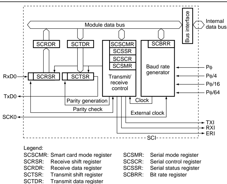
Figure 15.1 Smart Card Interface Block Diagram
