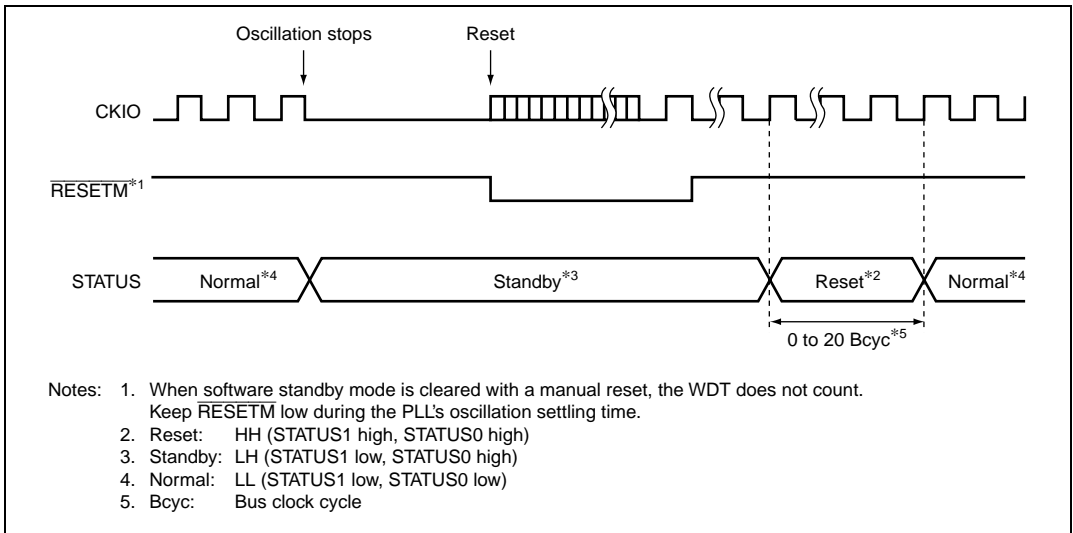
Figure 22.6 Software Standby to Manual Reset STATUS Output
