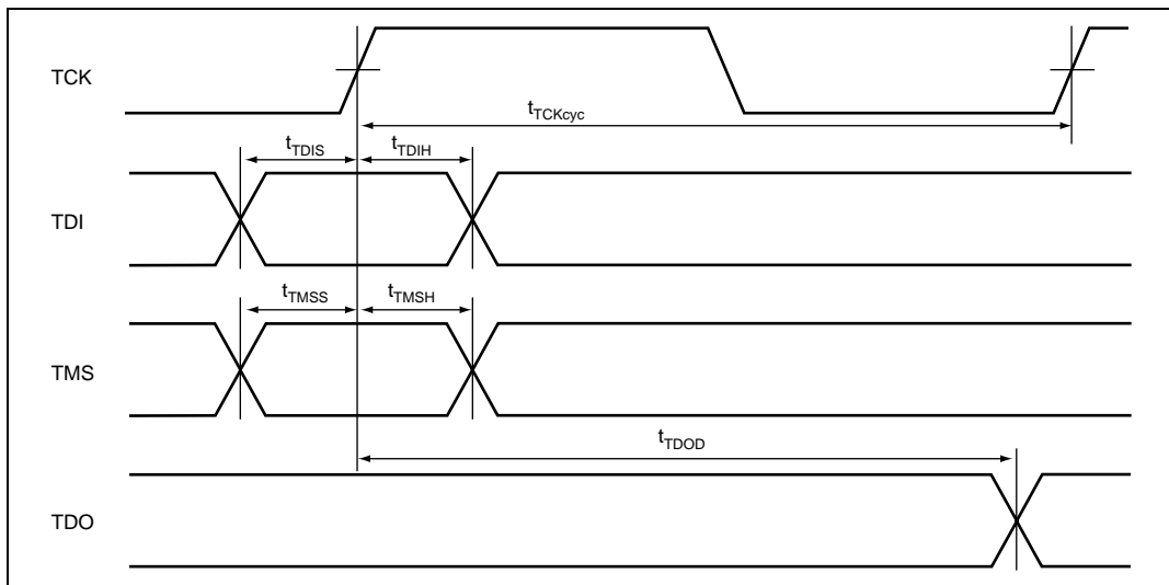
Figure 24.57 H-UDI Data Transfer Timing
