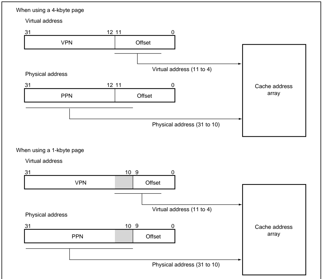
Figure 3.9 Synonym Problem
