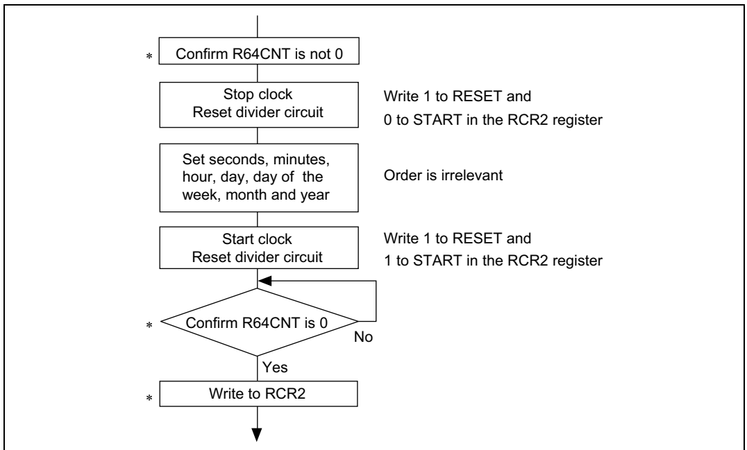
Figure 13.2(b) Setting the Time
