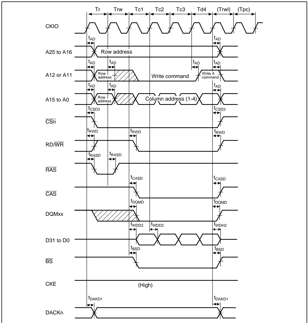
Figure 24.29 Synchronous DRAM Write Bus Cycle (Burst Mode (Single Write \times 4 ), RCD = 1, TPC = 0, TRWL = 0)
