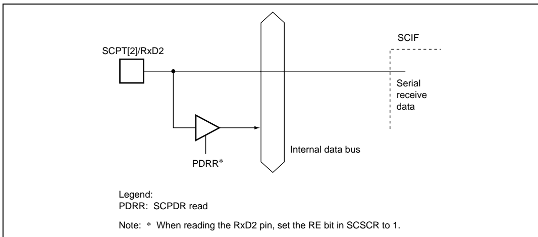
Figure 16.4 SCPT[2]/RxD2 Pin
