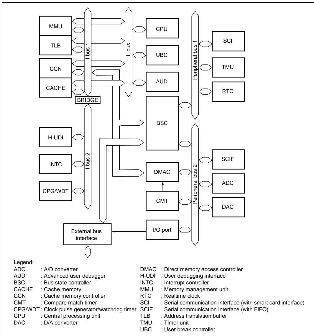
Figure 1.1 SH7706 Block Diagram
