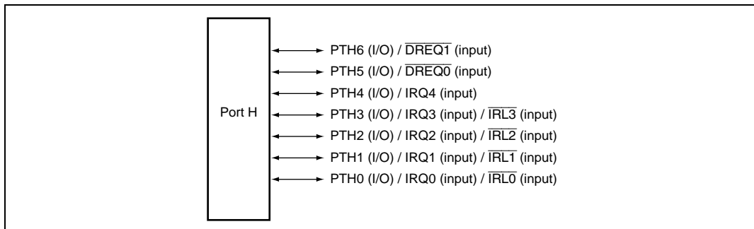
Figure 18.8 Port H
