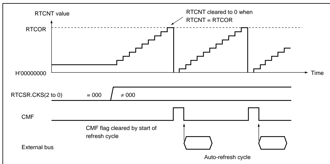
Figure 8.24 Auto-Refresh Operation
