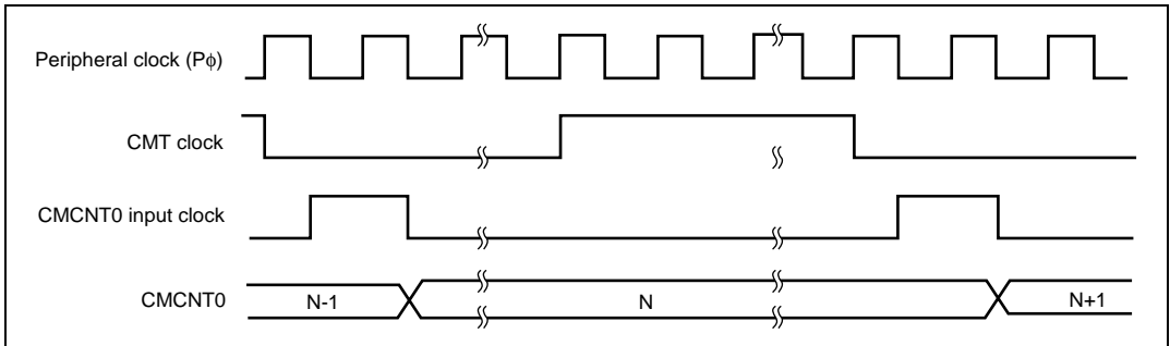
Figure 9.28 Count Timing
