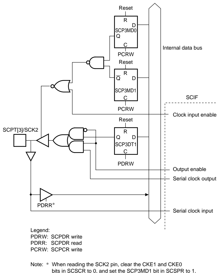
Figure 16.2 SCPT[3]/SCK2 Pin
