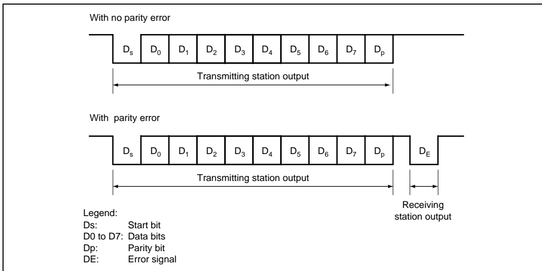
Figure 15.3 Data Format for Smart Card Interface
