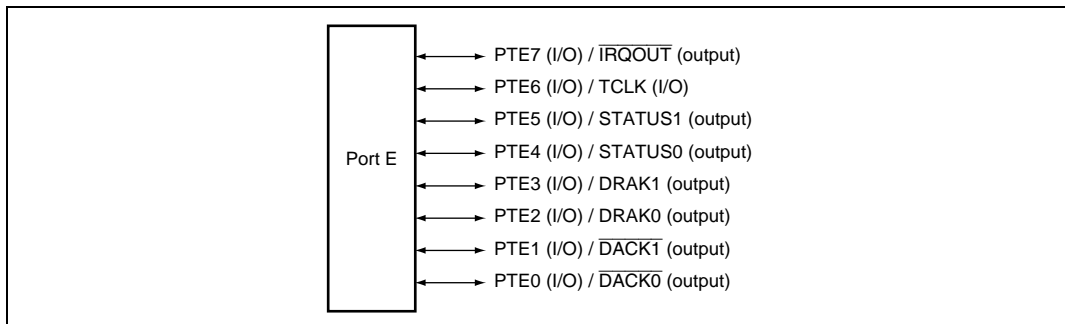
Figure 18.5 Port E
