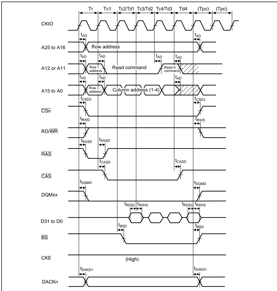
Figure 24.24 Synchronous DRAM Read Bus Cycle (Burst Read (Single Read \times 4), RCD = 0, CAS Latency = 1, TPC = 1)
