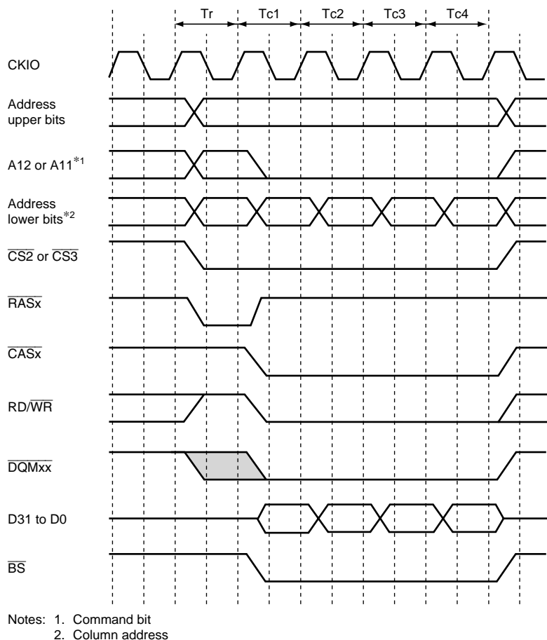
Figure 8.21 Burst Write Timing (No Precharge)
