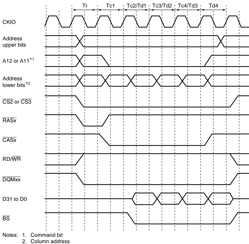
Figure 8.18 Burst Read Timing (No Precharge)
