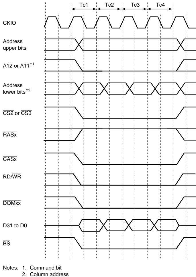
Figure 8.22 Burst Write Timing (Same Row Address)
