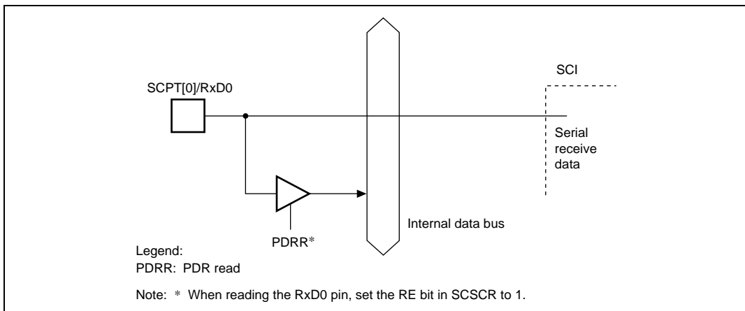
Figure 14.4 SCPT[0]/RxD0 Pin
