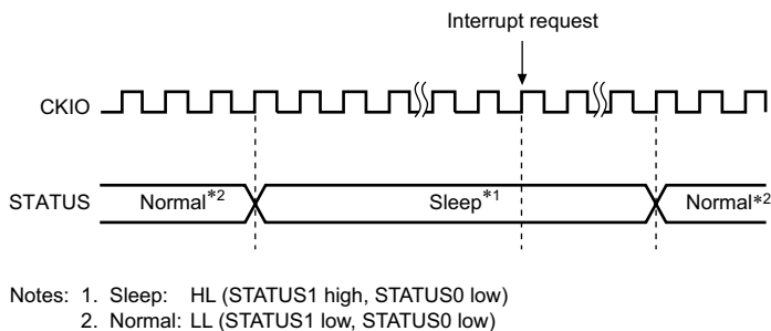
Figure 11.7 Canceling Sleep by Interrupt STATUS Output
