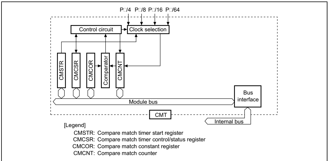
Figure 13.1 CMT Block Diagram
