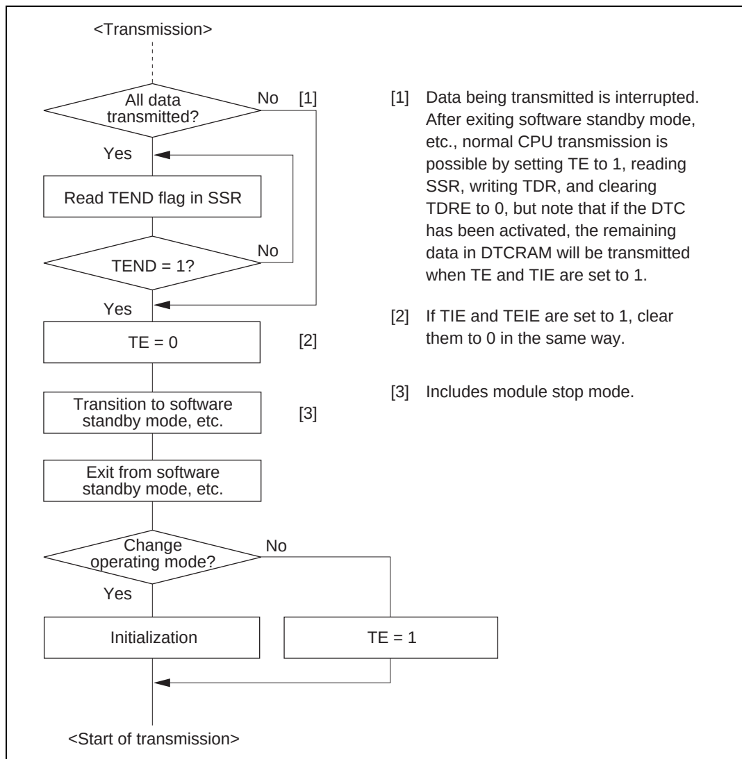
Figure 14.23 Sample Flowchart for Mode Transition during Transmission
