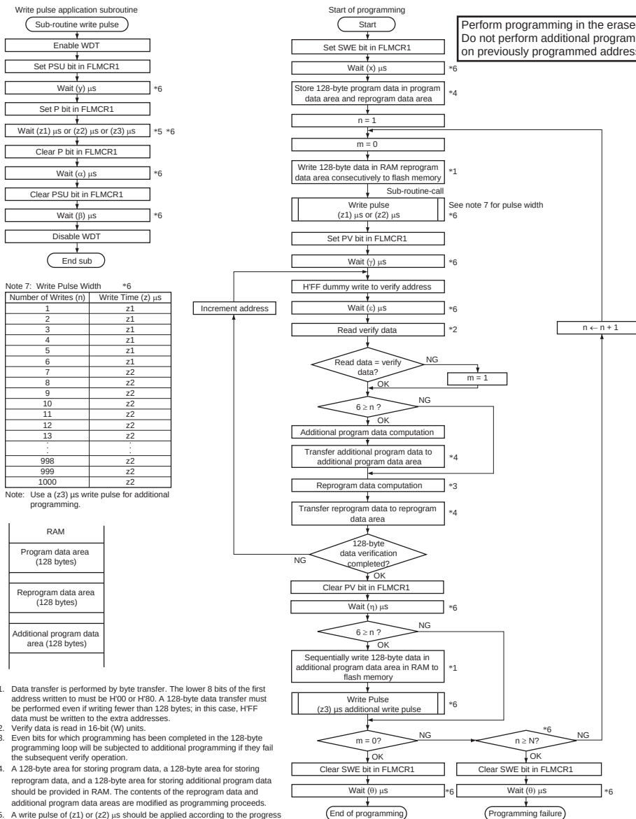
Program Data Operation Chart
