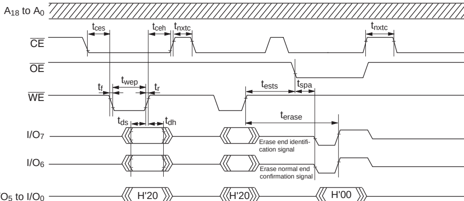
Figure 19.26 Auto-Erase Mode Timing Waveforms
