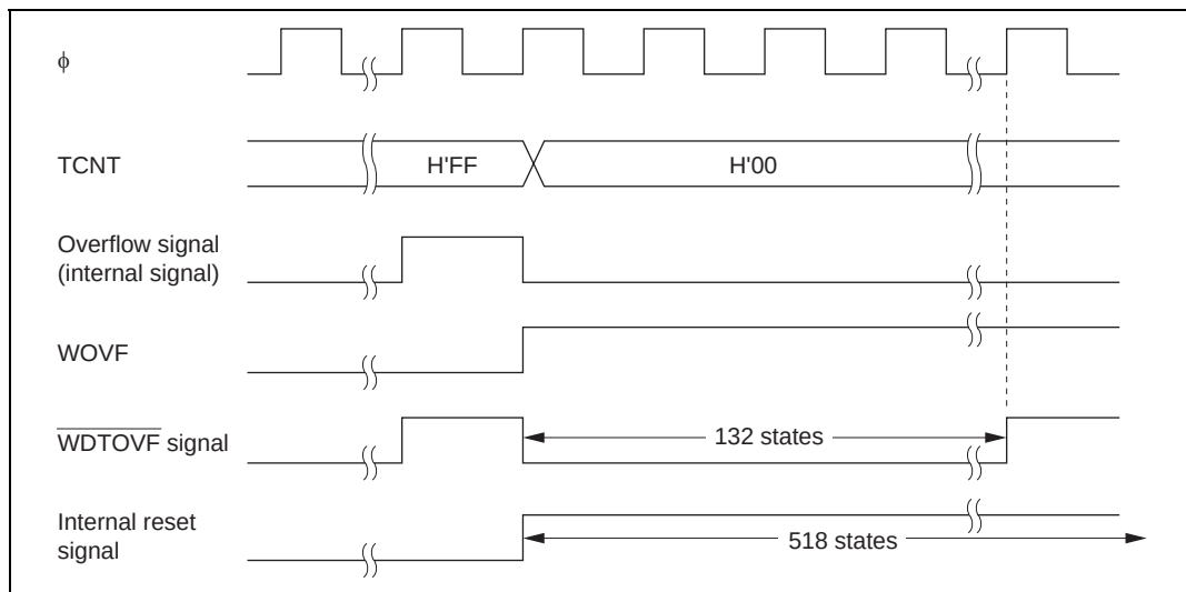
Figure 13.7 Timing of WOVF Setting
