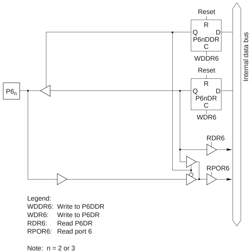
Figure C.6 (b) Port 6 Block Diagram (Pins P6 2 and P6 3 )
