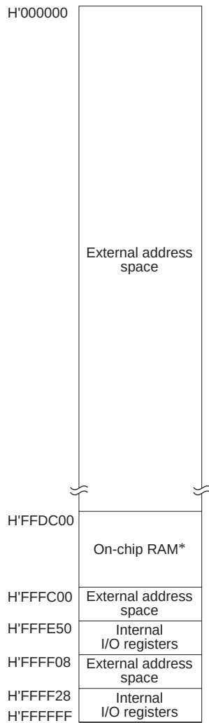
Figure 3.4 H8S/2332 Memory Map in Each Operating Mode
