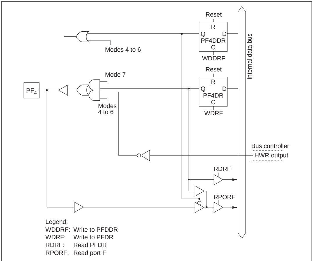
Figure C.15 (e) Port F Block Diagram (Pin PF 4 )
