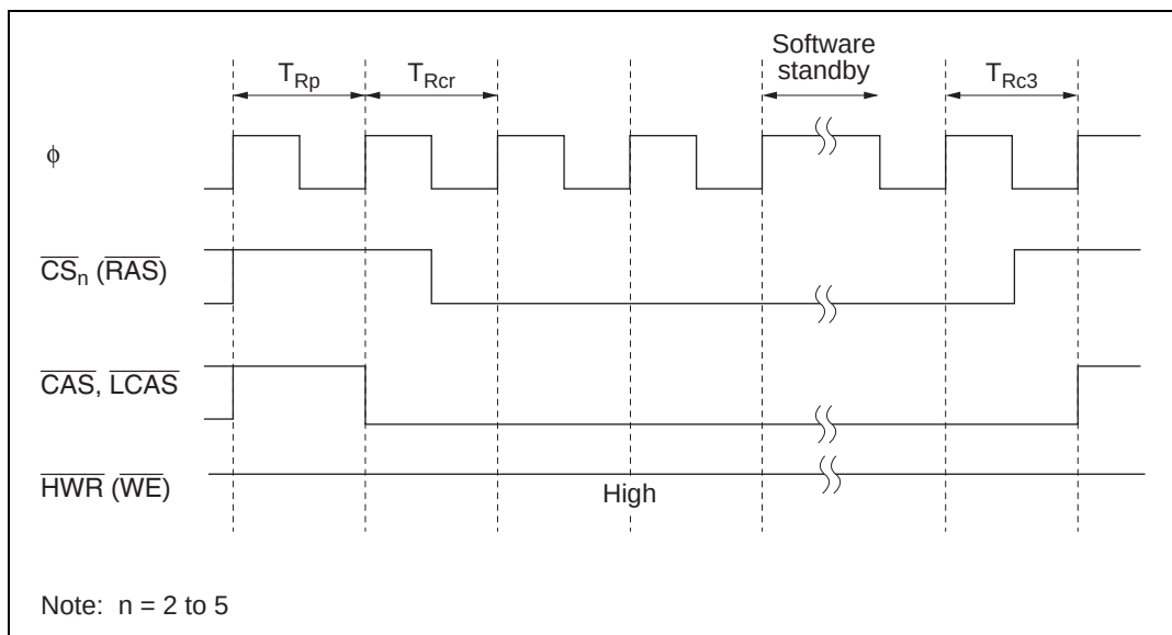
Figure 6.27 Self-Refresh Timing
