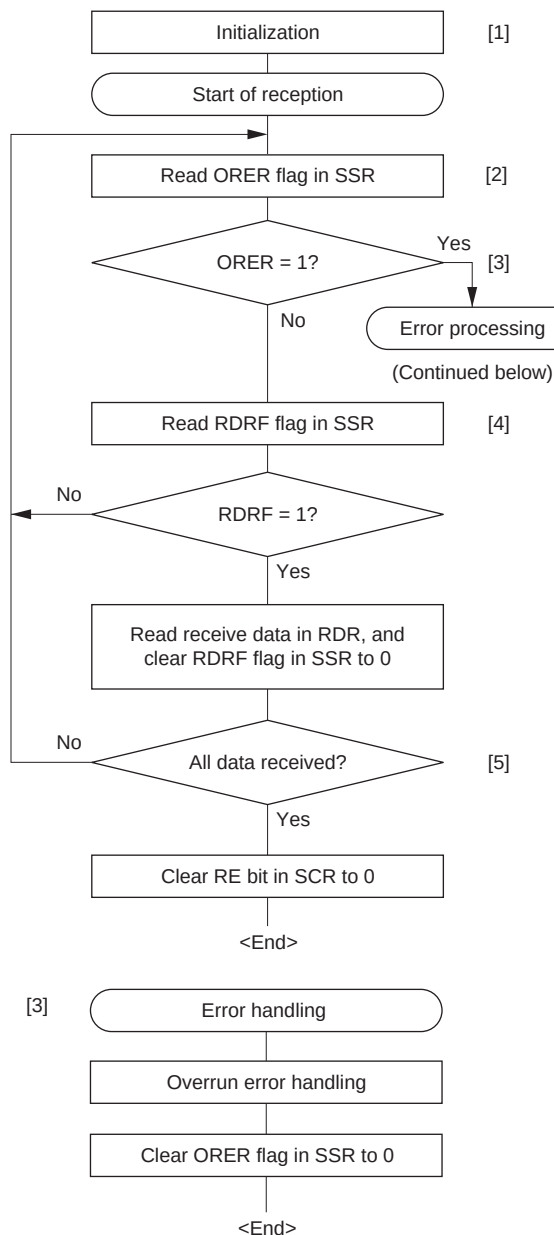
Figure 14.18 Sample Serial Reception Flowchart
