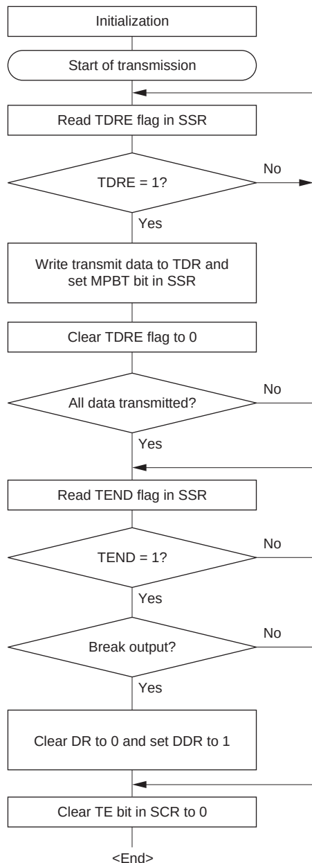
Figure 14.10 Sample Multiprocessor Serial Transmission Flowchart
