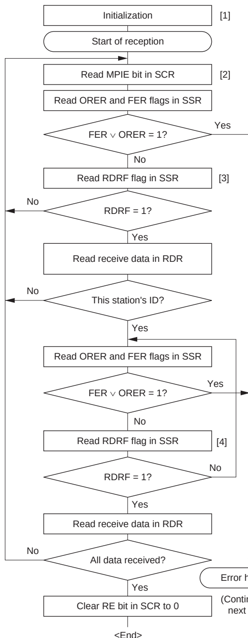
Figure 14.12 Sample Multiprocessor Serial Reception Flowchart
