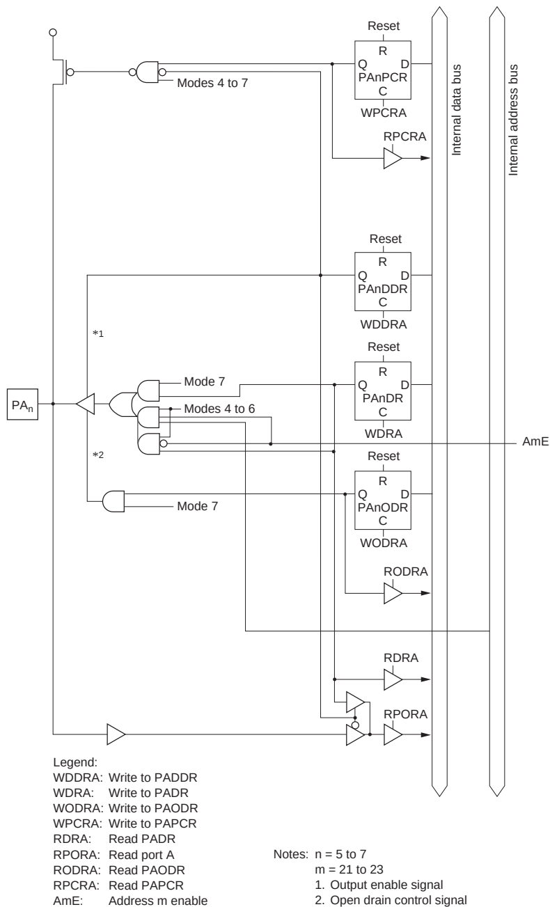
Figure C.10 (c) Port A Block Diagram (Pins PA 5 to PA 7 )
