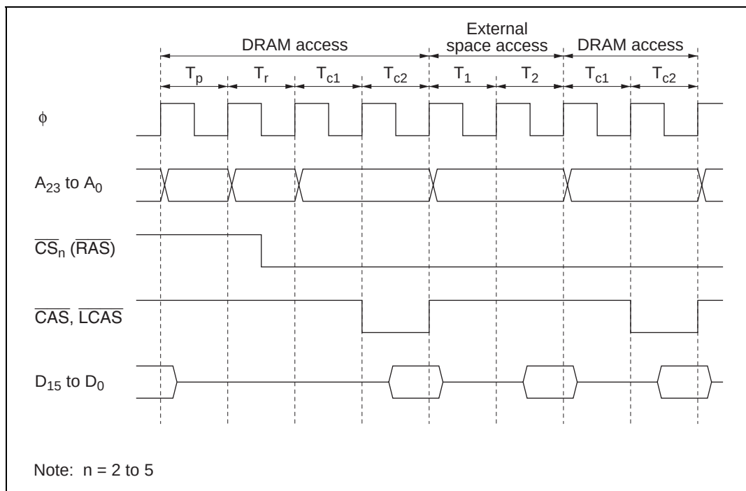
Figure 6.21 Example of Operation Timing in RAS Down Mode
