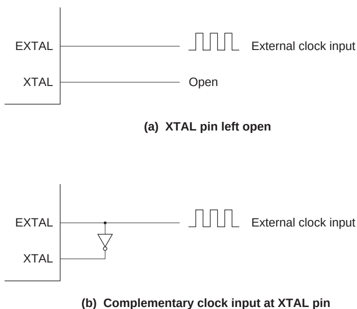
Figure 20.5 External Clock Input (Examples)
