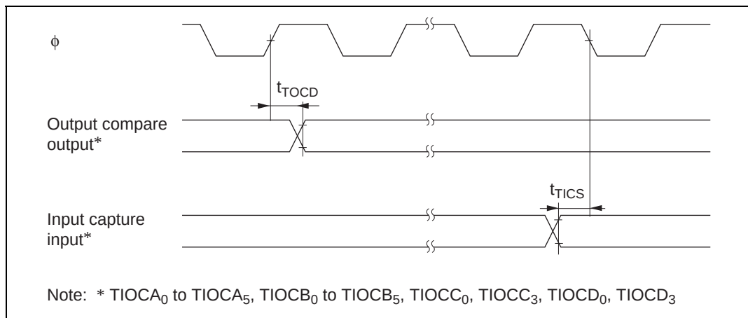
Figure 22.22 TPU Input/Output Timing
