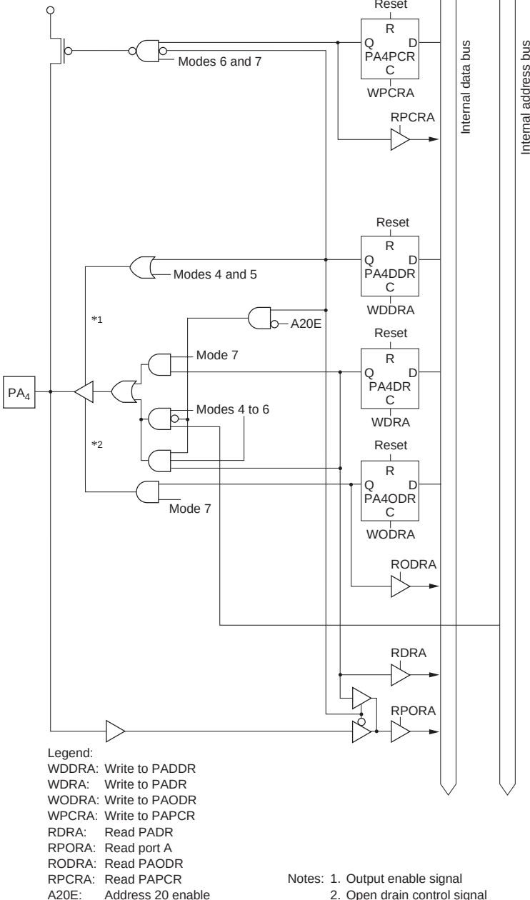
Figure C.10 (b) Port A Block Diagram (Pin PA 4 )
