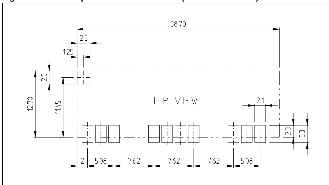
Figure 7. PCB footprint for GS-R12FSxxx1.9 (dimensions in mm)
