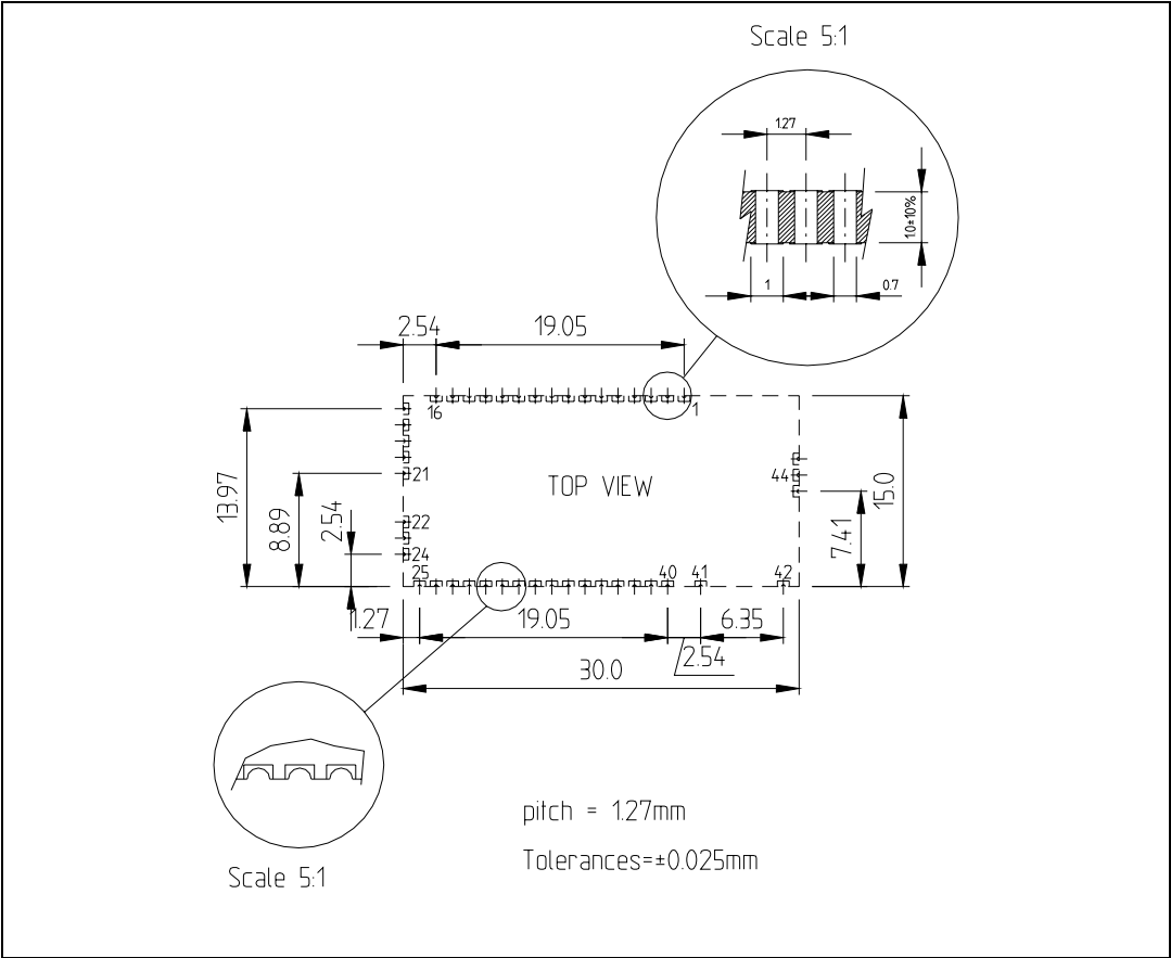
Figure 9. Mechanical dimensions
