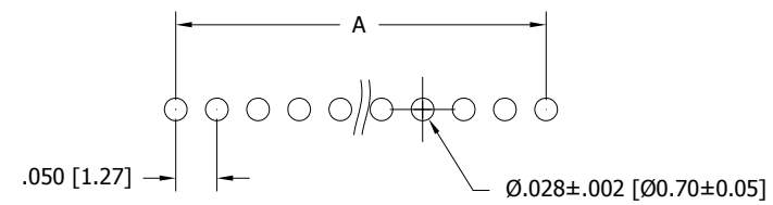
RECOMMENDED P.C. BOARD HOLE LAYOUT
