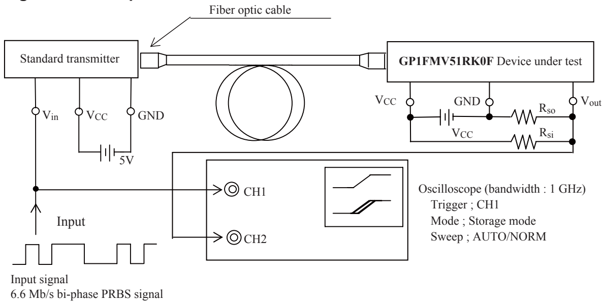
Fig. 4 Pulse Response and Jitter
