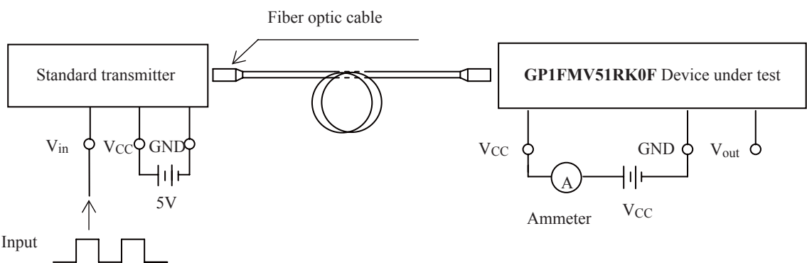
Fig. 1 Supply Current
