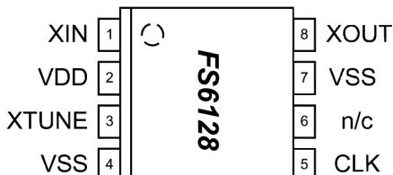
8-pin (0.150") SOIC
