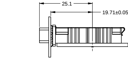
RECOMMENDED FACE PLATE TO LOCATING POST DISTANCE
