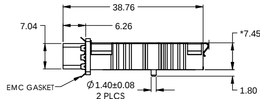
RECOMMENDED FACE PLATE TO LOCATING POST DISTANCE
