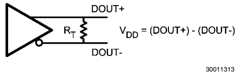
FIGURE 10. Serializer V_{OD} Diagram
