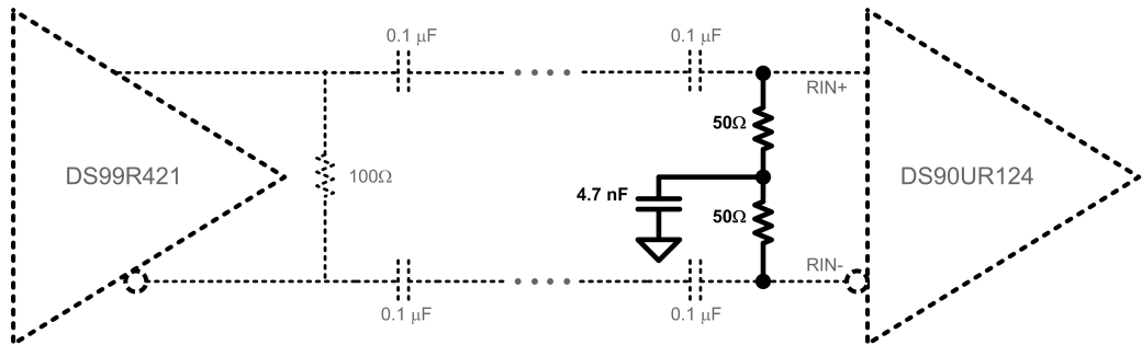
FIGURE 14. Receiver Termination Option 2
