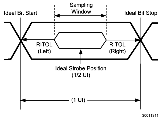
FIGURE 8. Receiver RITOL Left and Right
