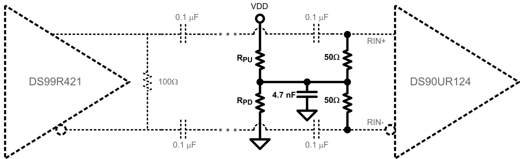
FIGURE 15. Receiver Termination Option 3
