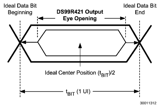
FIGURE 9. Serializer Output Eye Opening
