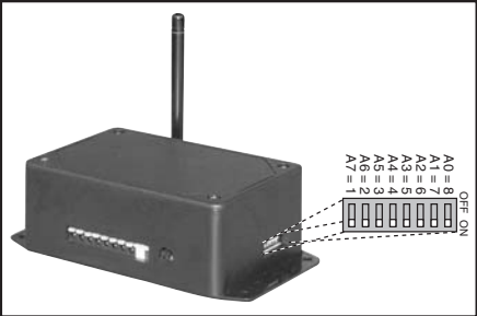
Figure 4: Address DIP Switches
