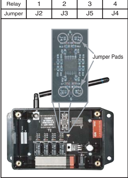
Figure 3: Jumper Pad Locations
