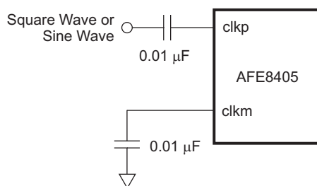
Figure 6-8. AC-Coupled, Single-Ended Clock Input
