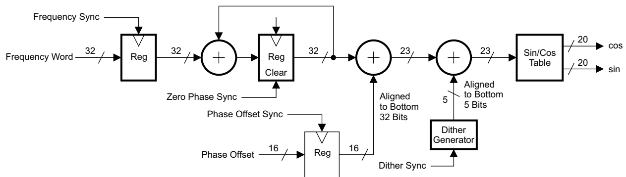
Figure 7-16. Detailed NCO Circuit
