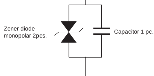
[Equivalent Circuit]
