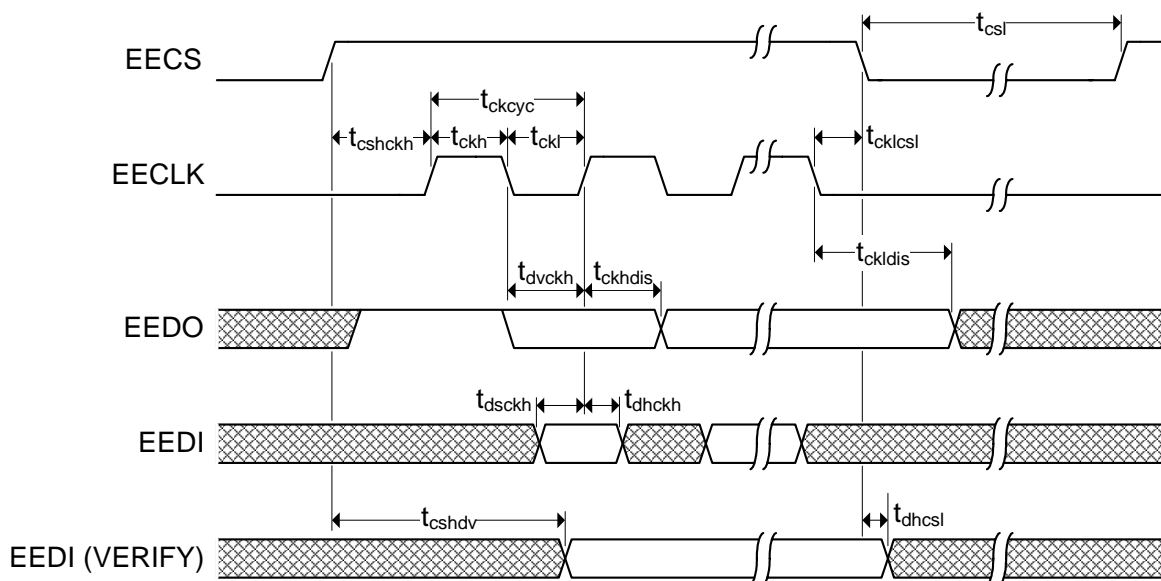
Figure 15.10 Microwire Timing
