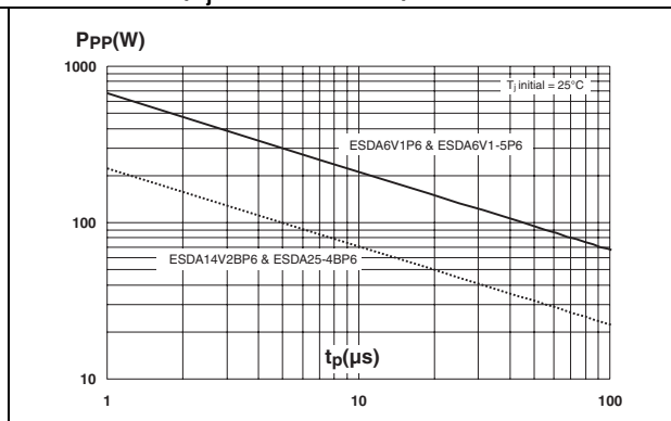
Figure 5. Peak pulse power versus exponential pulse duration ( T_j \text{ initial} = 25^\circ\text{C} )
