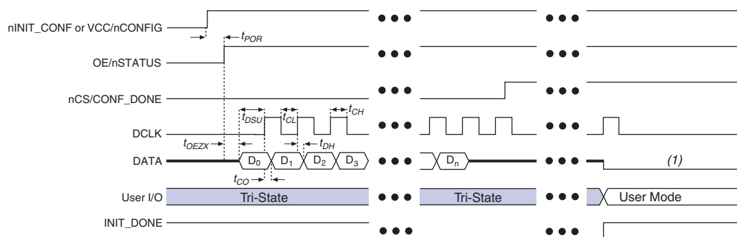
Figure 5-5. Timing Waveform Using a Configuration Device
