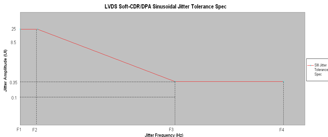
Figure 1–2. Stratix III LVDS Soft-CDR/DPA Sinusoidal Jitter Tolerance Spec
