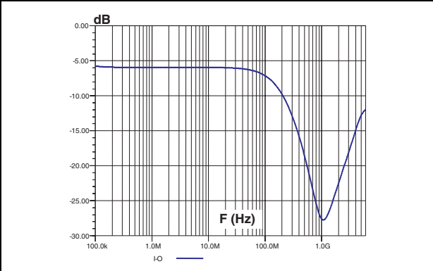
Figure 3. S21 attenuation measurement ( V_{bias} = 0\text{ V} )
