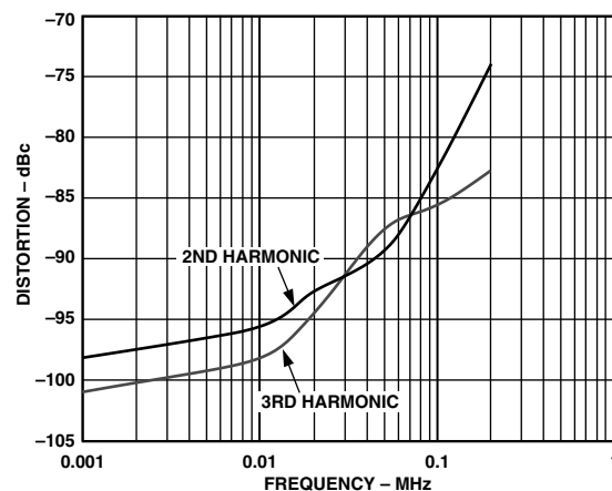
TPC 12. Distortion vs. Frequency, V_S = \pm 12\text{ V} , R_L = 600\ \Omega , V_{OUT} = 20\text{ V p-p}
