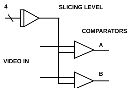
FIGURE 14. DELAY DETECTOR
