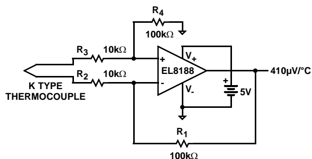
FIGURE 31. THERMOCOUPLE AMPLIFIER
