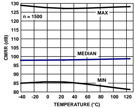
FIGURE 22. CMRR vs TEMPERATURE, V_+ = \pm 2.5V, \pm 1.5V
