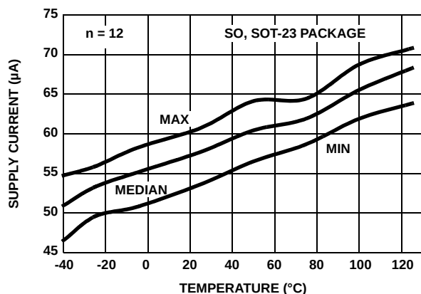
FIGURE 25. SUPPLY CURRENT vs TEMPERATURE V_S = \pm 2.5V ENABLED. R_L = \text{INF}
