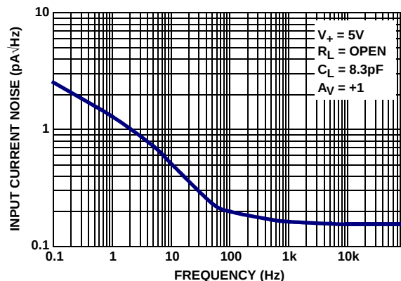
FIGURE 16. INPUT CURRENT NOISE DENSITY vs FREQUENCY
