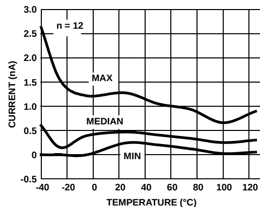
FIGURE 31. I_{BIAS}(-) vs TEMPERATURE V_S = \pm 1.2V
