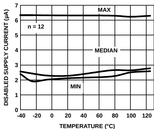
FIGURE 27. DISABLED SUPPLY CURRENT vs TEMPERATURE V_S = \pm 2.5V R_L = INF
