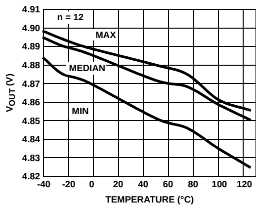
FIGURE 42. POSITIVE V_{OUT} vs TEMPERATURE R_L = 1k V_S = \pm 2.5V
