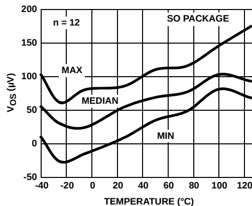
FIGURE 34. INPUT OFFSET VOLTAGE vs TEMPERATURE V_S = \pm 2.5V
