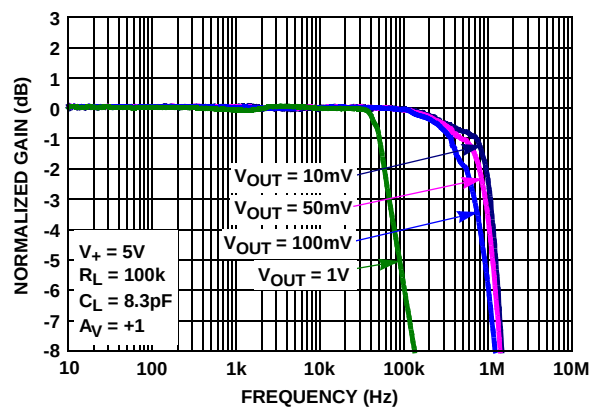
FIGURE 6. GAIN vs FREQUENCY vs V_{OUT} , R_L = 100k
