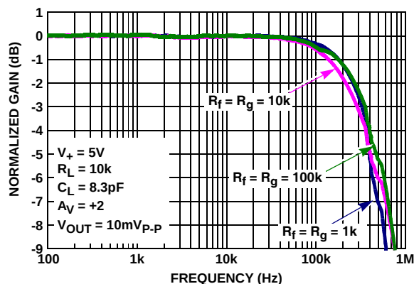
FIGURE 3. GAIN vs FREQUENCY vs FEEDBACK RESISTOR VALUES R_f/R_g
