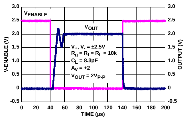
FIGURE 20. ENABLE TO OUTPUT RESPONSE
