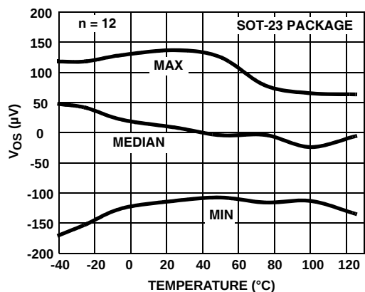
FIGURE 37. INPUT OFFSET VOLTAGE vs TEMPERATURE V_S = \pm 1.2V
