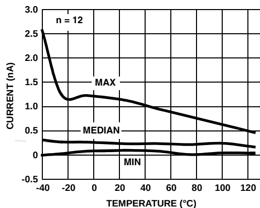
FIGURE 29. I_{BIAS}(+) vs TEMPERATURE V_S = \pm 1.2V
