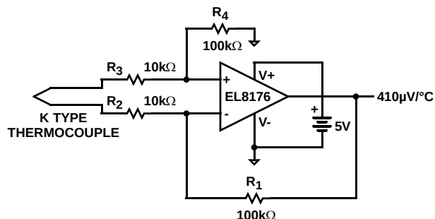
FIGURE 51. THERMOCOUPLE AMPLIFIER
