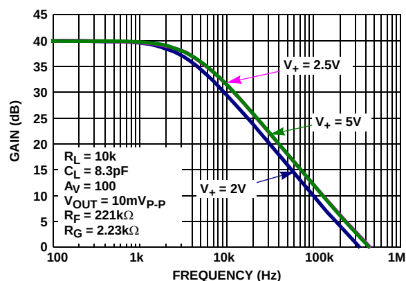
FIGURE 10. GAIN vs FREQUENCY vs SUPPLY VOLTAGE
