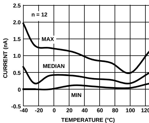
FIGURE 30. I_{BIAS}(-) vs TEMPERATURE V_S = \pm 2.5V
