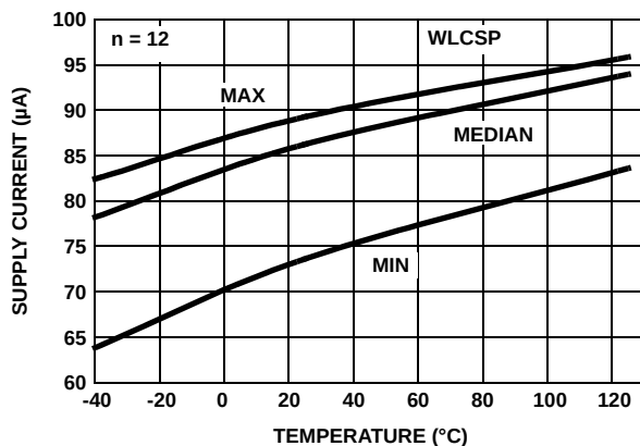
FIGURE 26. SUPPLY CURRENT vs TEMPERATURE V_S = \pm 2.5V ENABLED. R_L = \text{INF}
