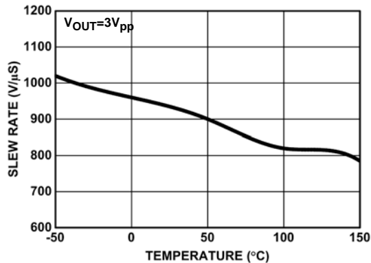
FIGURE 29. SLEW RATE vs TEMPERATURE
