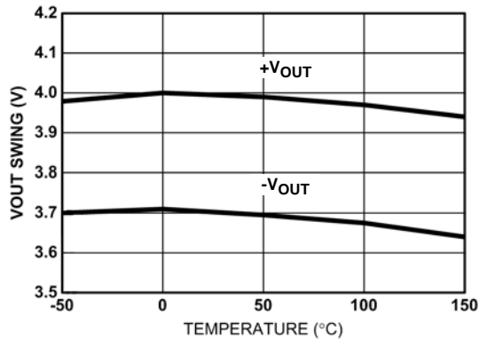
FIGURE 25. OUTPUT SWING vs TEMPERATURE
