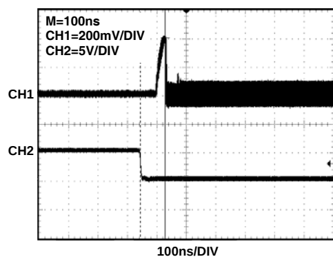
FIGURE 19. ENABLED RESPONSE
