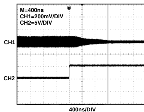
FIGURE 20. DISABLED RESPONSE
