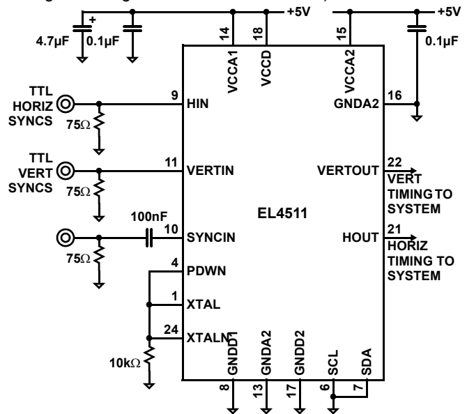
FIGURE 8. APPLICATIONS DRAWING 1
