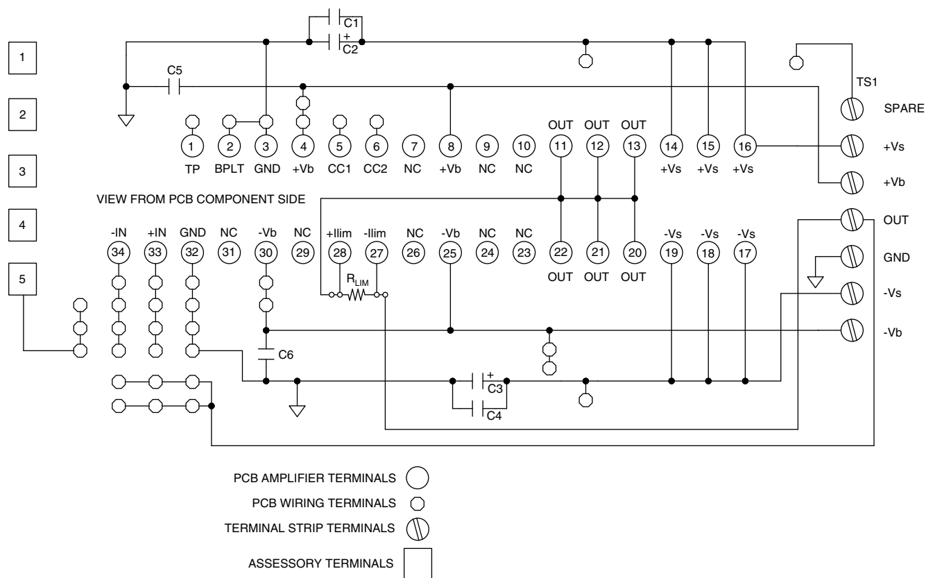
FIGURE 1: SCHEMATIC DIAGRAM
