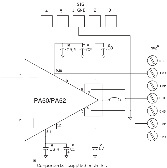
FIGURE 2. PCB SCHEMATIC.
