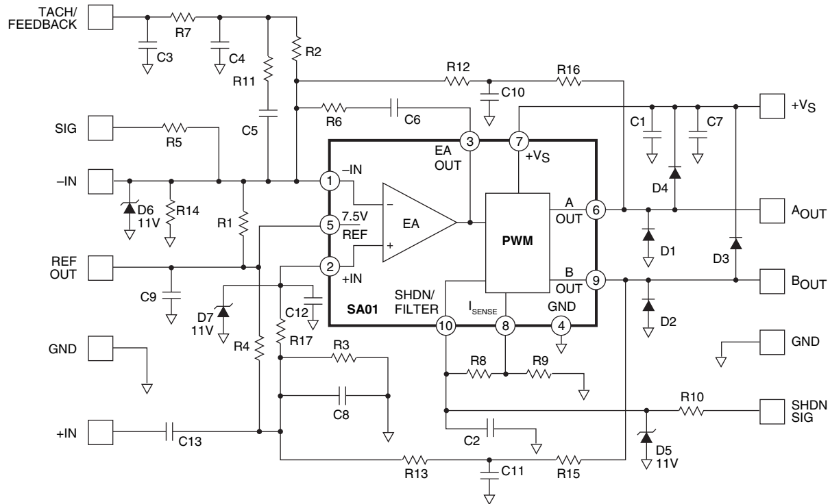
FIGURE 2. PCB SCHEMATIC.
