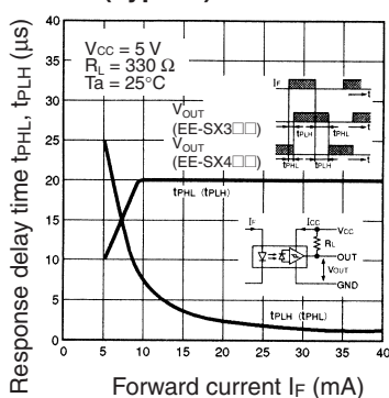
Response Delay Time vs. Forward Current (Typical)
