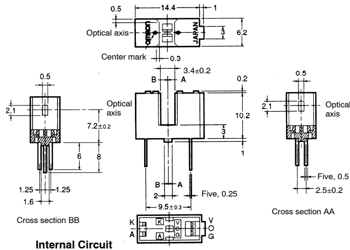
Internal Circuit
