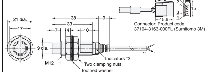
Diagram 10 E2E-X8MD□ E2E-X5ME□/F□ Pre-wired e-CON Connector Models
