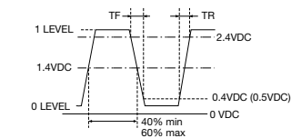
Figure 2) TTL Output Wave Form
