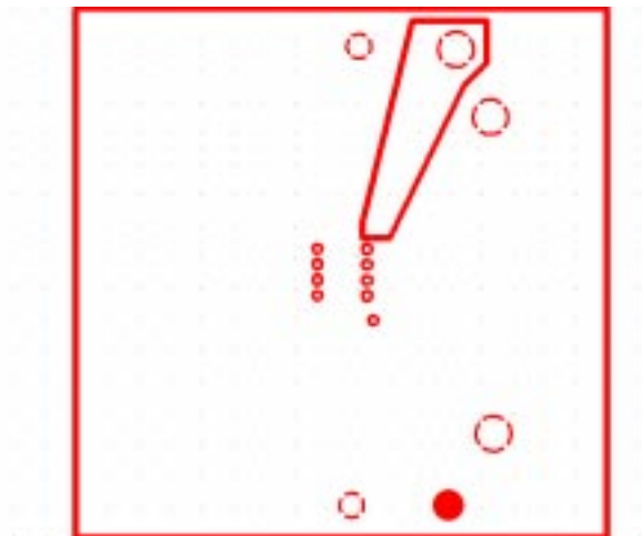
Third Layer (VCC and Ground Plane)
