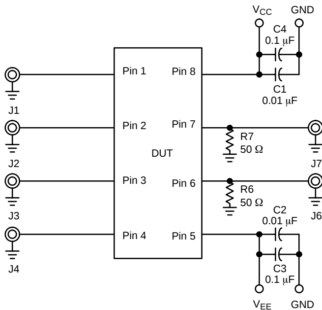
Figure 6. Configuration 3 Schematic
