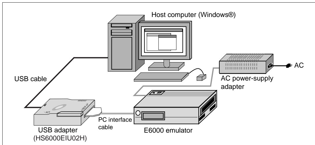
Figure 1.1 System Configuration of E6000 Emulator Connection
